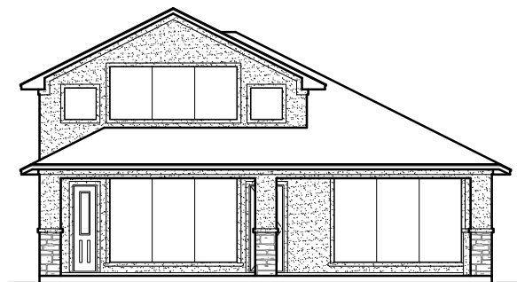
Rear Elevation ③
