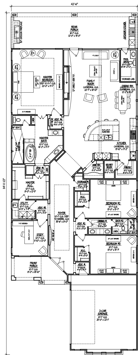
Architectural 1st Floor Plan ①
