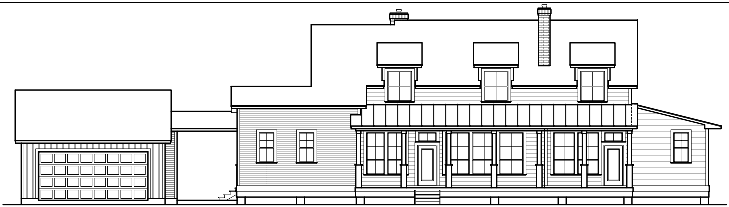
Rear Elevation 4
