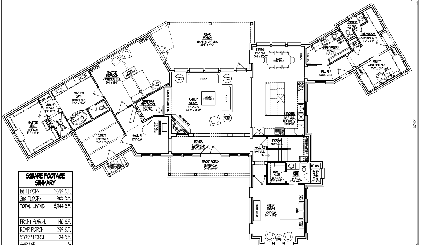
Architectural 1st Floor Plan ③
