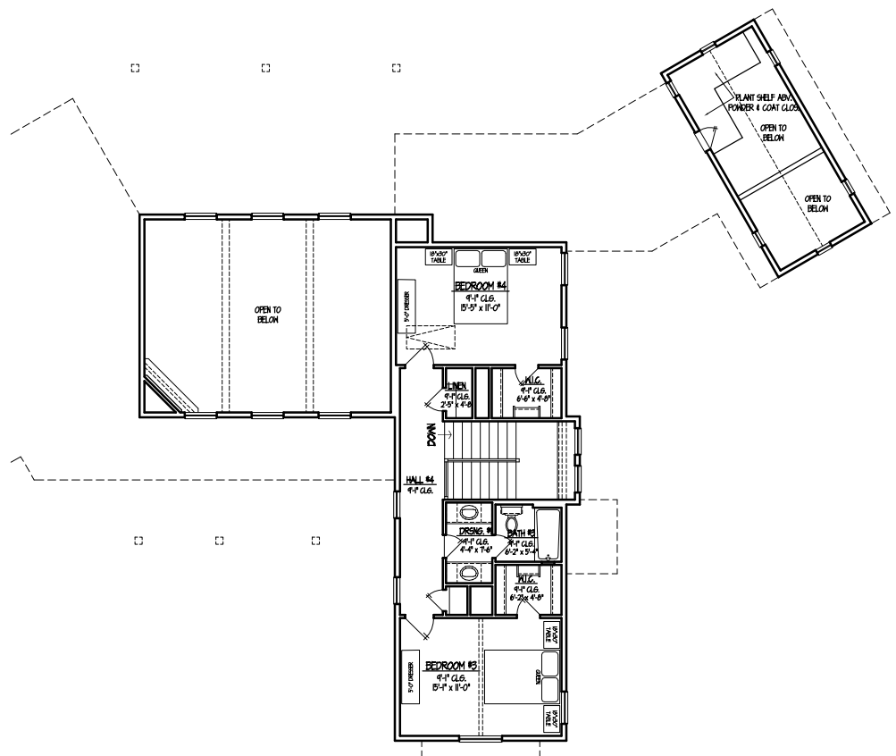
Architectural 2nd Floor Plan
