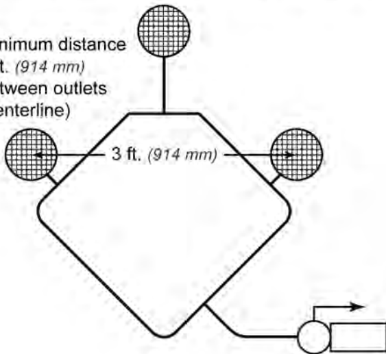
Figure 14. Three or more outlets in parallel, looped piping
