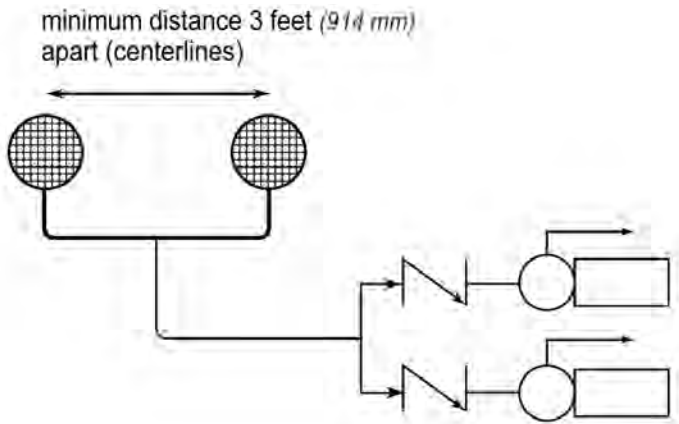
Figure 10. Dual outlets in parallel to dual pumps
