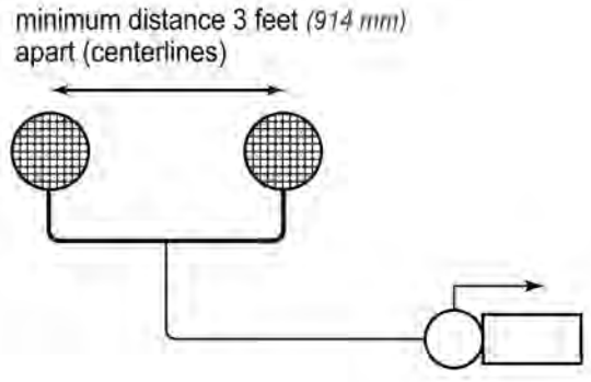
Figure 9. Dual outlets in parallel to one pump
