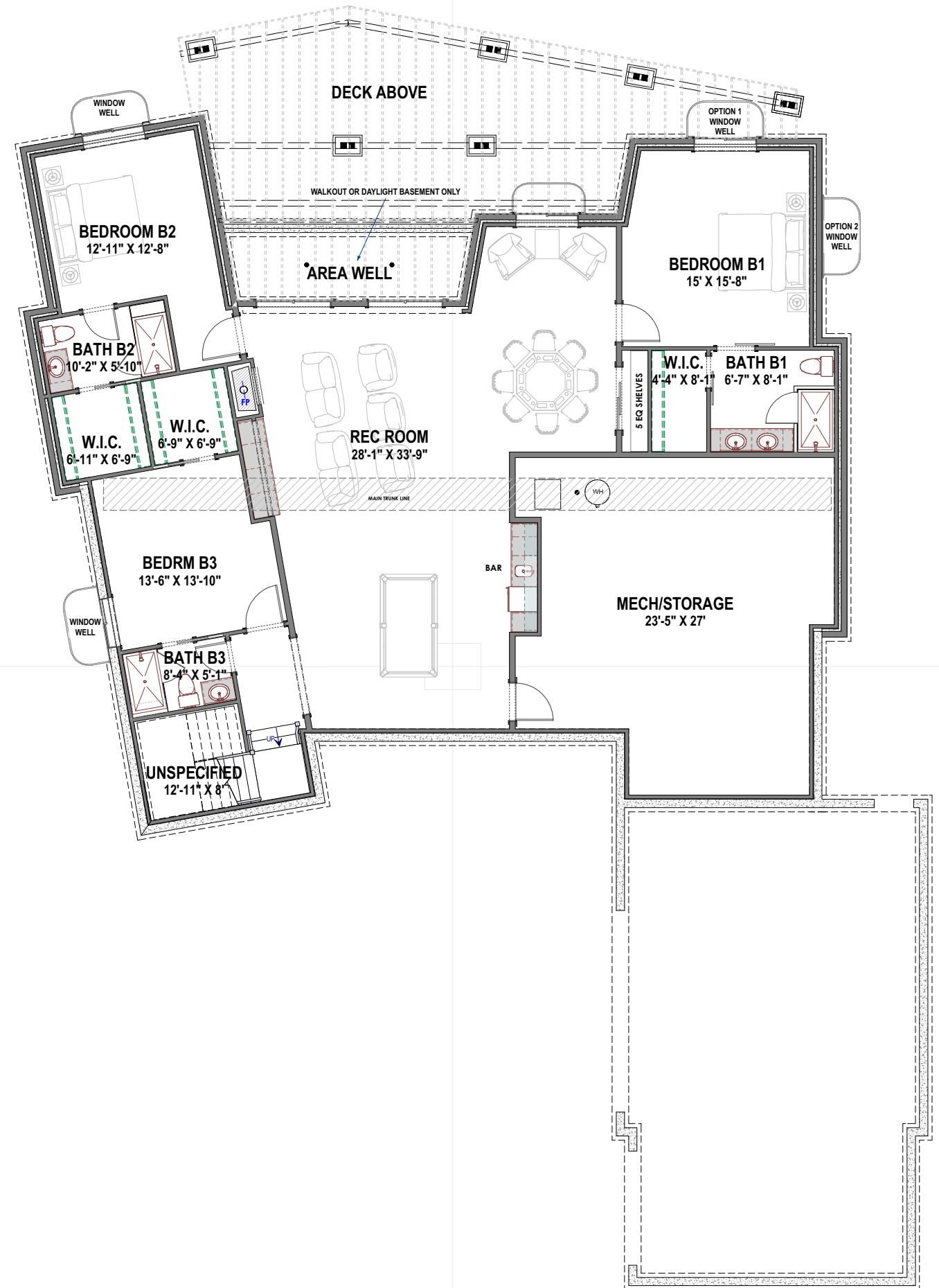
BASEMENT LEVEL 3/32"=1'-0"
