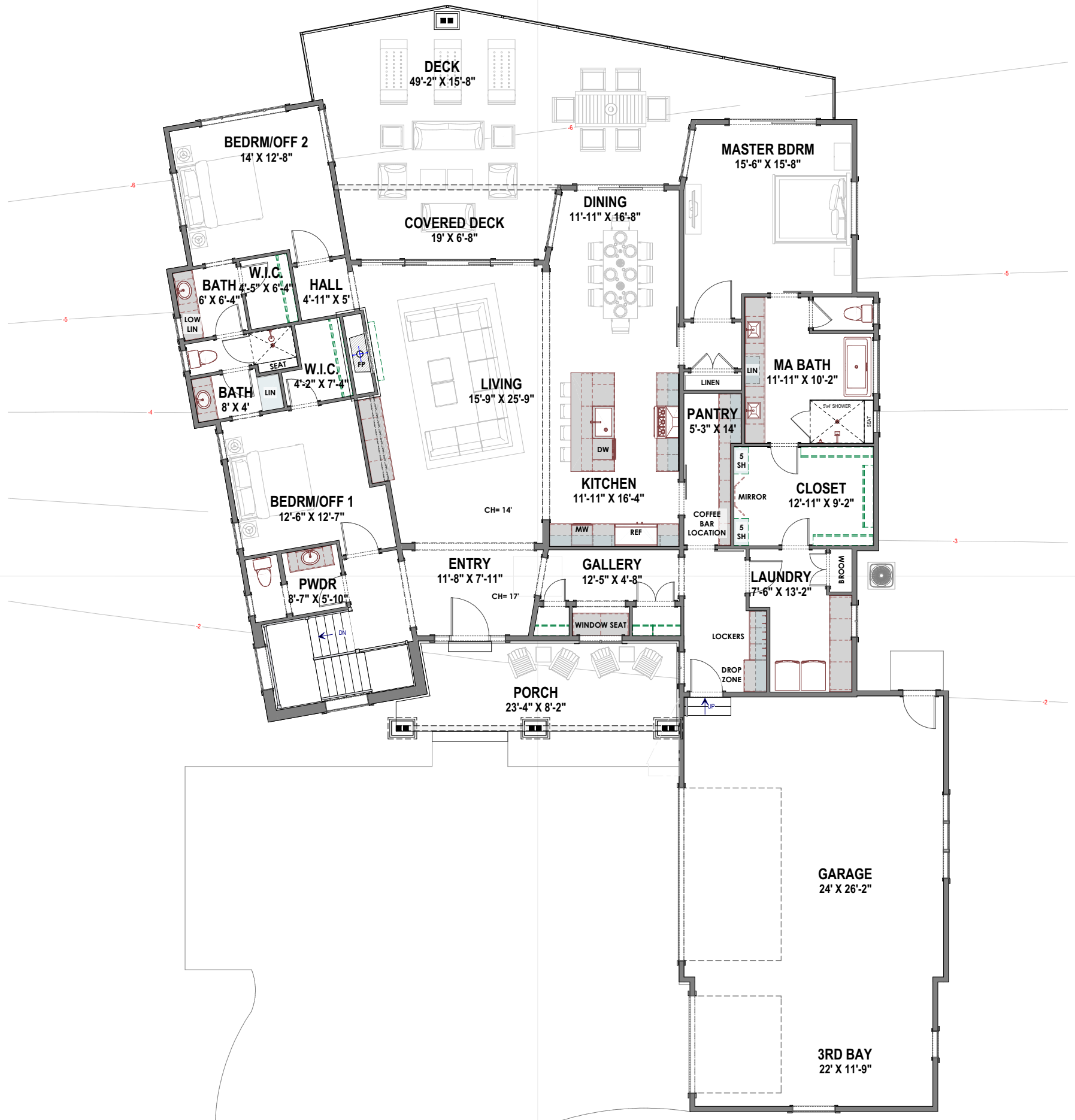
MAIN LEVEL 3/32"=1'-0"
