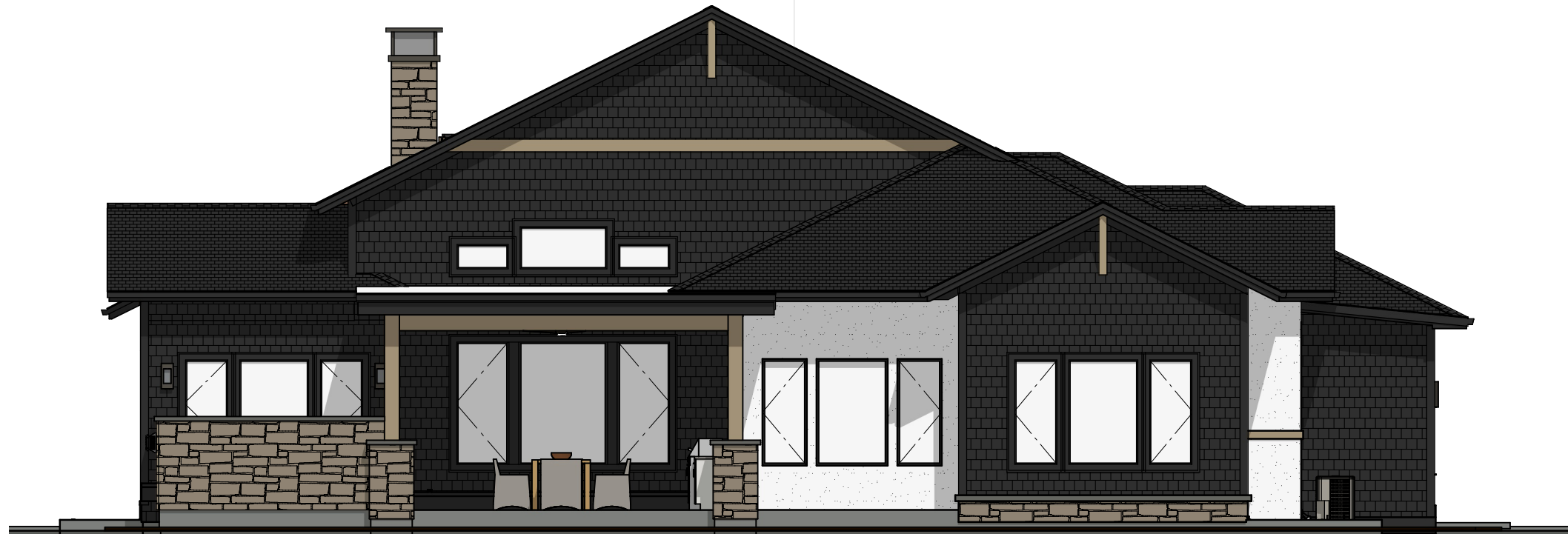
BACK ELEVATION
