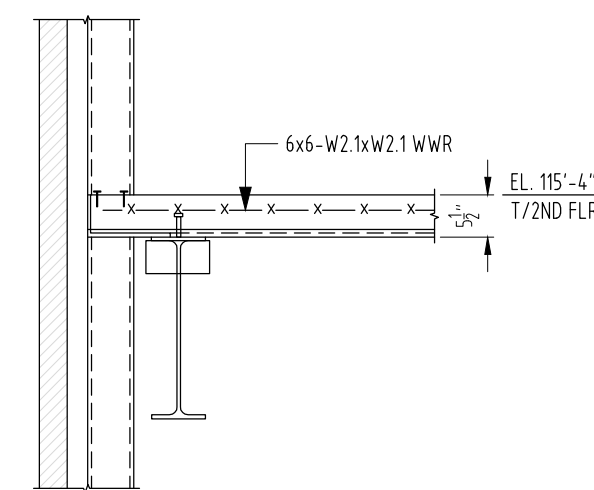
SECTION 5 SCALE: 1/2"=1'-0" SDR: 11/S5.66
