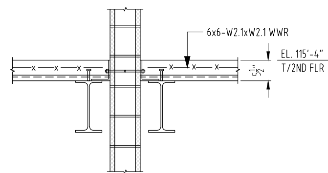
SECTION 8 SCALE: 1/2"=1'-0" SDR: 95M/55.64
