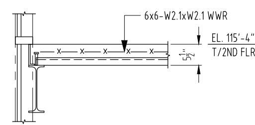
SECTION SCALE: 1/2"=1'-0" SDR: 12/S5.64
