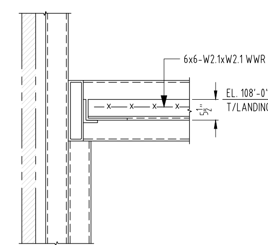
SECTION SCALE: 1/2"=1'-0" SDR: 2/S3.02 & 5/S3.02
