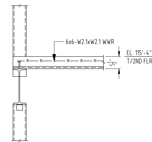
SECTION SCALE: 1/2"=1'-0" SDR: 6/55.63
