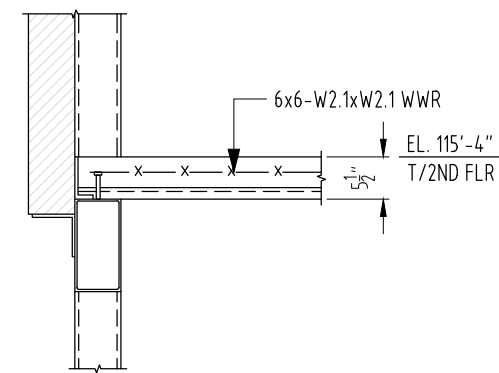
SECTION SCALE: 1/2"=1'-0" SDR: 8/S5.64
