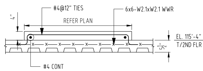
SECTION 13 SCALE: 1/2"=1'-0" SDR: 13/55.61
