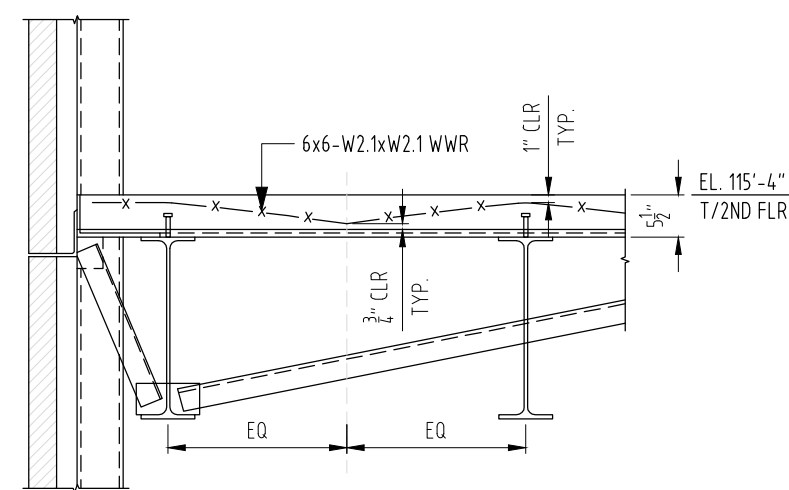
SECTION 1 SCALE: 1/2"=1'-0" SDR: 16/55.66
