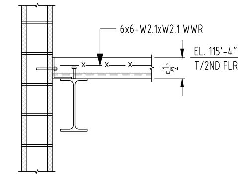
SECTION 6 SCALE: 1/2"=1'-0" SDR: 9/55.64
