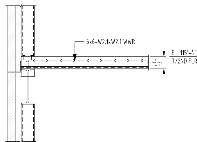
SECTION 2 SCALE: 1/2"=1'-0" SDR: 12/55.66
