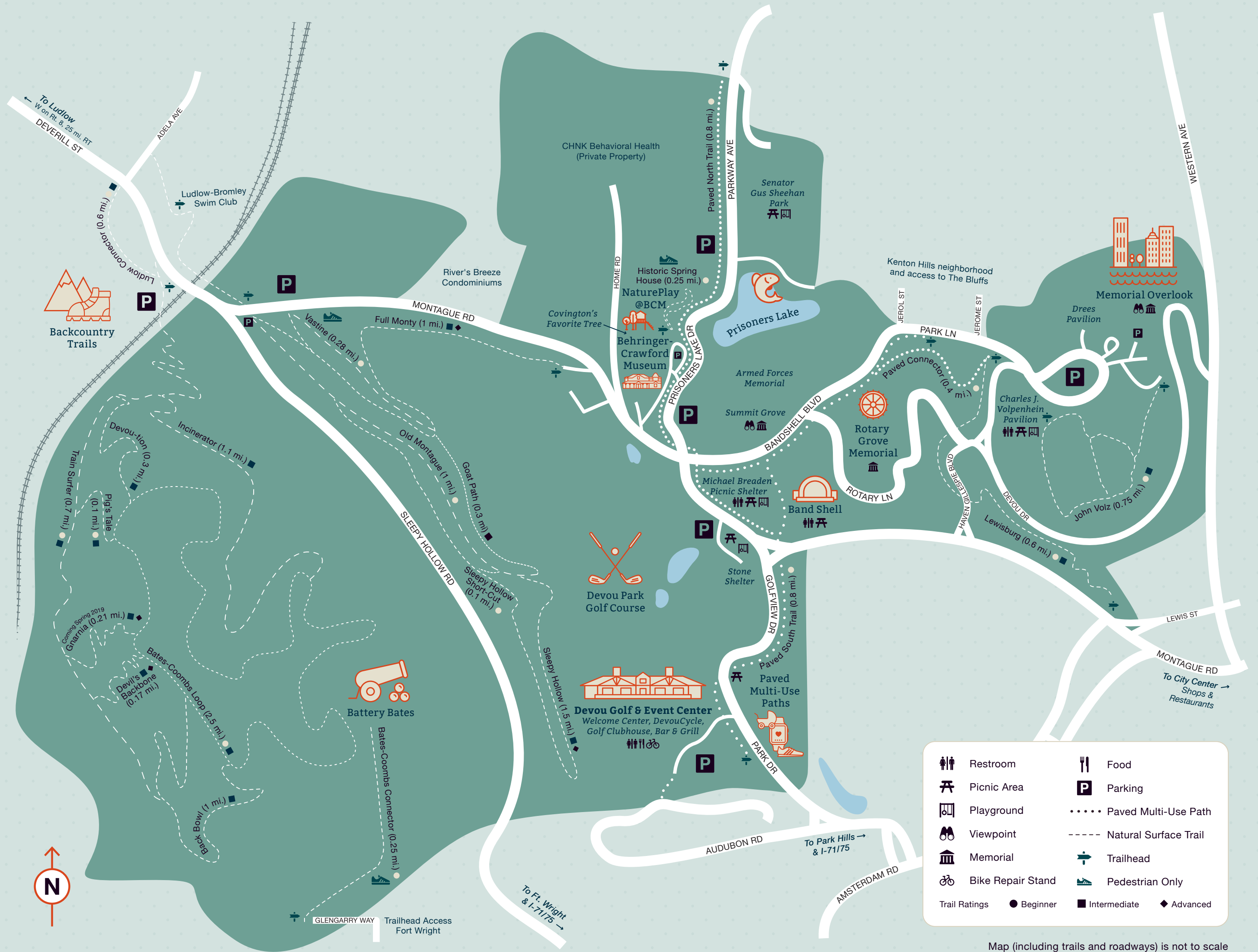
Map (including trails and roadways) is not to scale Effective through October 2019
