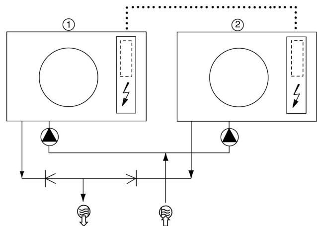
Configuration: leaving water control
