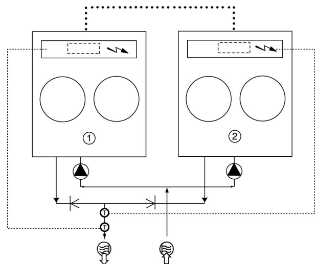
Configuration: leaving water control
