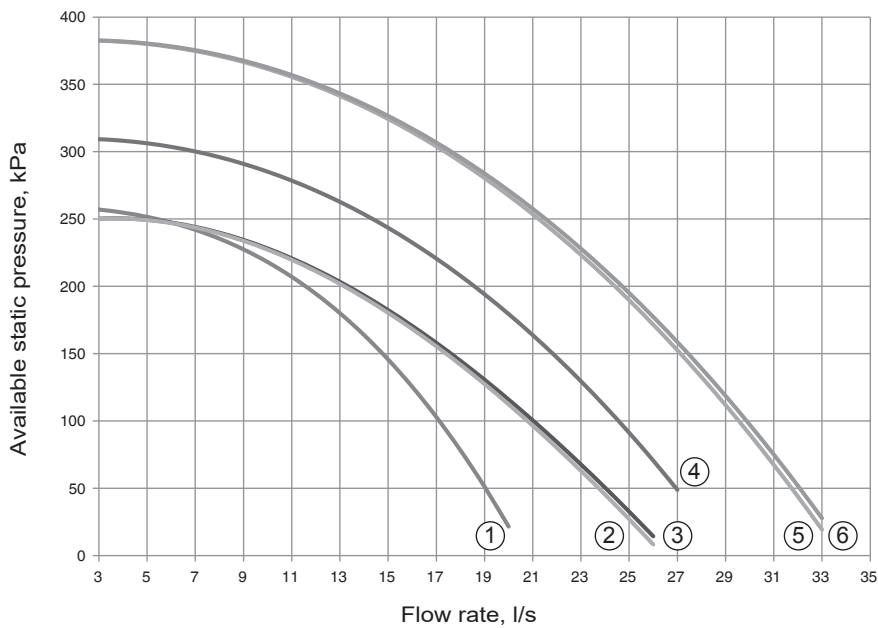
Single pumps
