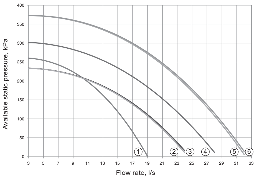
Dual pumps
