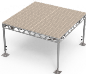
8' x 8' COMPLETE STANDING DOCK KIT 4' - 8' LEGS 255 lbs / 115 kg (w/o decking - 155 lbs / 70 kg)
