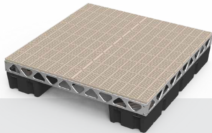
8' X 8' COMPLETE FLOATING DOCK KIT
