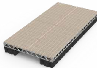
8' X 16' COMPLETE FLOATING DOCK KIT 650 lbs / 295 kg (w/o decking - 450 lbs / 204 kg)
