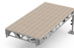
4' x 8' COMPLETE QUICK LINK DOCK KIT 2' - 4' LEGS 130 lbs / 59 kg (w/o decking - 80 lbs / 36 kg)
