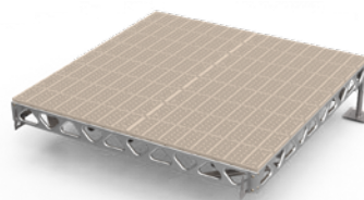
8' x 8' COMPLETE QUICK LINK DOCK KIT 1' - 2' LEGS 215 lbs / 98 kg (w/o decking - 115 lbs / 52 kg)
