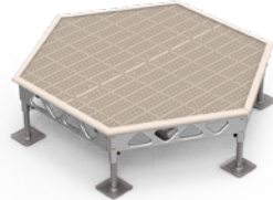
7' x 8' COMPLETE HEXAGON STANDING DOCK KIT 1' - 2' LEGS 205 lbs / 93 kg (w/o decking - 105 lbs / 47 kg)
