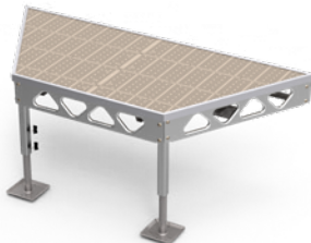
STANDING TRANSITION KIT 2' - 4' LEGS 110 lbs / 50 kg (w/o decking - 60 lbs / 27 kg)
