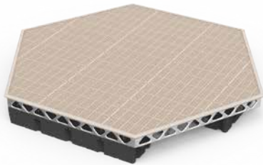
14' x 16' COMPLETE HEXAGON FLOATING DOCK KIT 860 lbs / 390 kg (w/o decking - 560 lbs / 254 kg)
