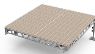
8' x 8' COMPLETE QUICK LINK DOCK KIT 2' - 4' LEGS 220 lbs / 100 kg (w/o decking - 120 lbs / 54 kg)
