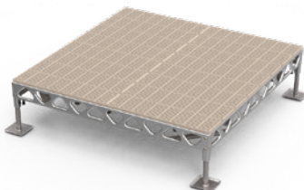
8' x 8' COMPLETE STANDING DOCK KIT 1' - 2' LEGS 225 lbs / 102 kg (w/o decking - 125 lbs / 57 kg)
