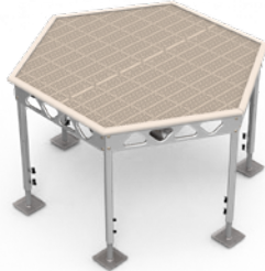
7' x 8' COMPLETE HEXAGON STANDING DOCK KIT 4' - 8' LEGS 250 lbs / 113 kg (w/o decking - 150 lbs / 68 kg)
