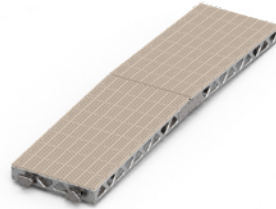
4' X 16' COMPLETE RAMP KIT 250 lbs / 114 kg (w/o decking - 150 lbs / 68 kg)
