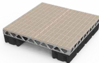
8' X 8' COMPLETE FLOATING DOCK KIT 315 lbs / 143 kg (w/o decking - 215 lbs / 98 kg)
