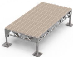
4' x 8' COMPLETE STANDING DOCK KIT 1' - 2' LEGS 135 lbs / 61 kg (w/o decking - 85 lbs / 39 kg)
