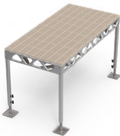
4' x 8' COMPLETE STANDING DOCK KIT 4' - 8' LEGS 165 lbs / 75 kg (w/o decking - 115 lbs / 52 kg)
