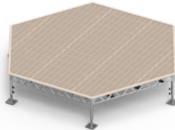
14' x 16' COMPLETE HEXAGON STANDING DOCK KIT 2' - 4' LEGS 625 lbs / 283 kg (w/o decking - 325 lbs / 147 kg)
