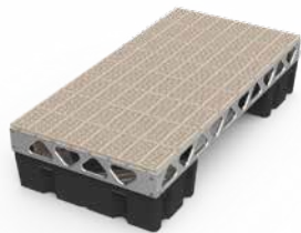
4' X 8' COMPLETE FLOATING DOCK KIT 175 lbs / 79 kg (w/o decking - 125 lbs / 57 kg)
