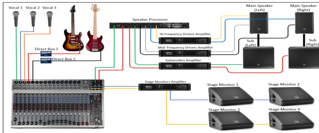
Figure PA3- “The Passive PA System”
