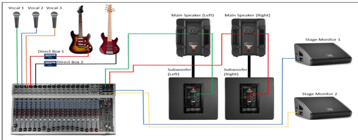
Figure PA2- "The Active PA System"
