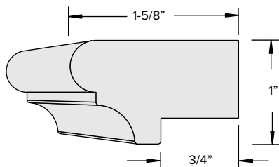
CR1 Chair Rail1- 3/4" Cap (not to scale)
