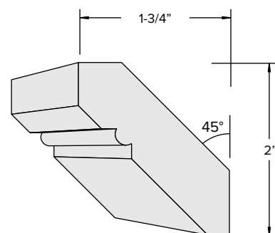
Crown5 2-7/8" Beaded Shaker Crown Pattern
