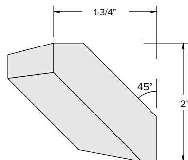
Crown4 2-7/8" Shaker Crown Pattern
