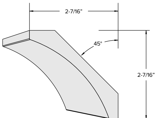
Crown9 3-1/2" Crown Pattern
