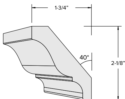
Crown2 2-3/4" Crown Pattern
