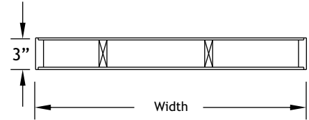
Island Boxed End Panel
