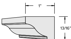
Canopy Moulding 1 1" Crown Pattern
