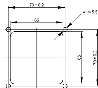
取付用穴加工図 Panel arrangements
