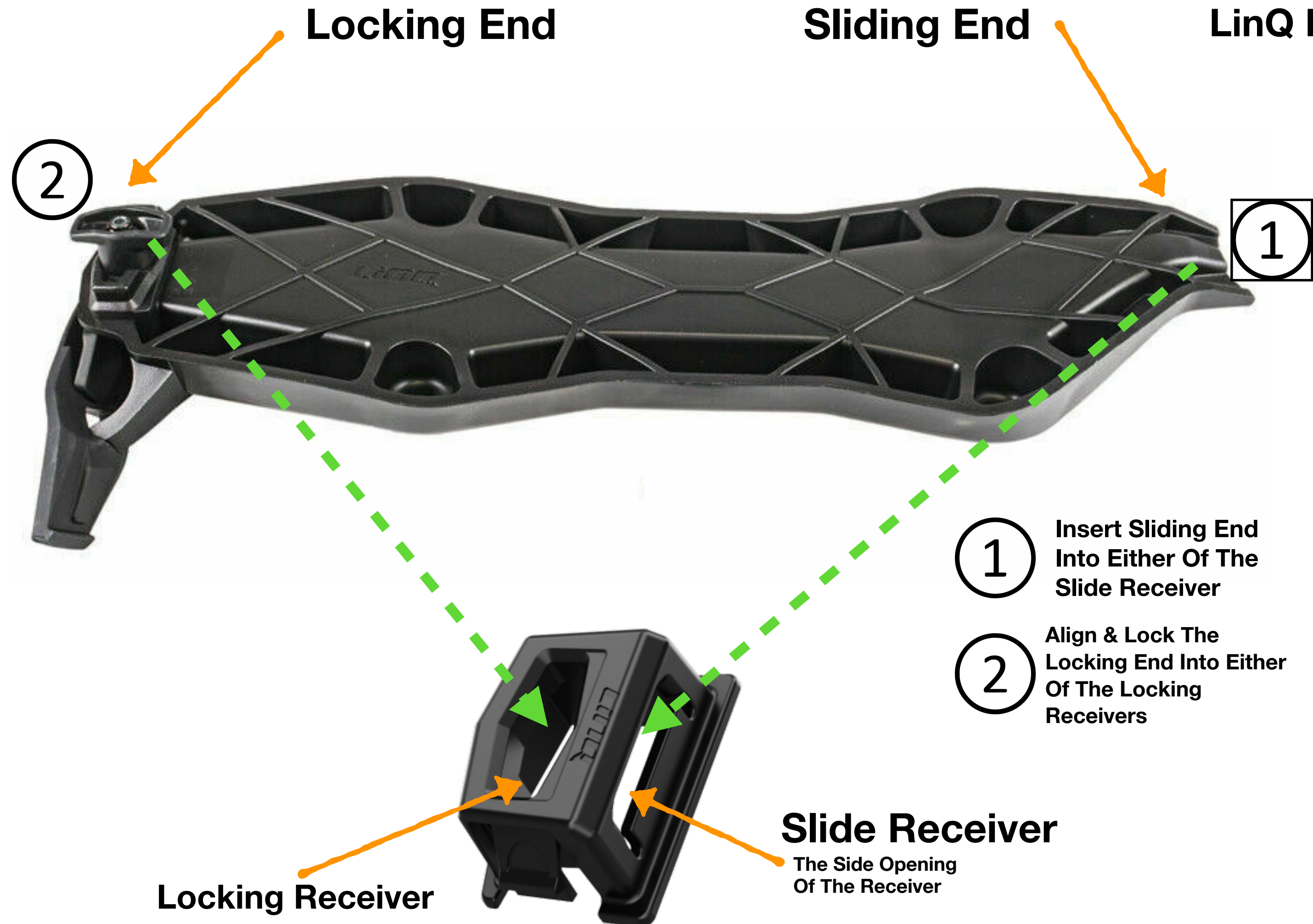
LinQ Receivers Open/Locked Position
