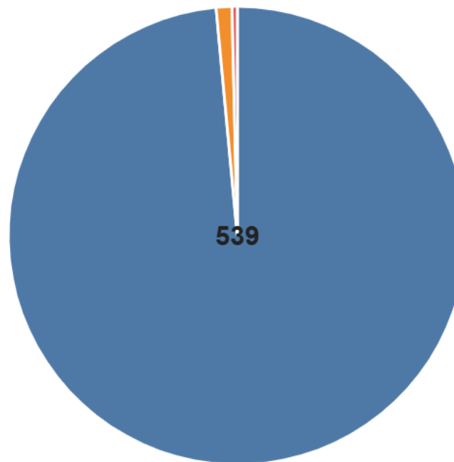
Class Counts
