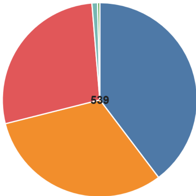
Category Counts
