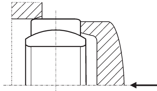
Figure 4: Installation tool
