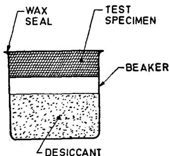
FIG. 2 ARRANGEMENT OF SPECIMEN FOR WATER VAPOUR PERMEANCE TEST
