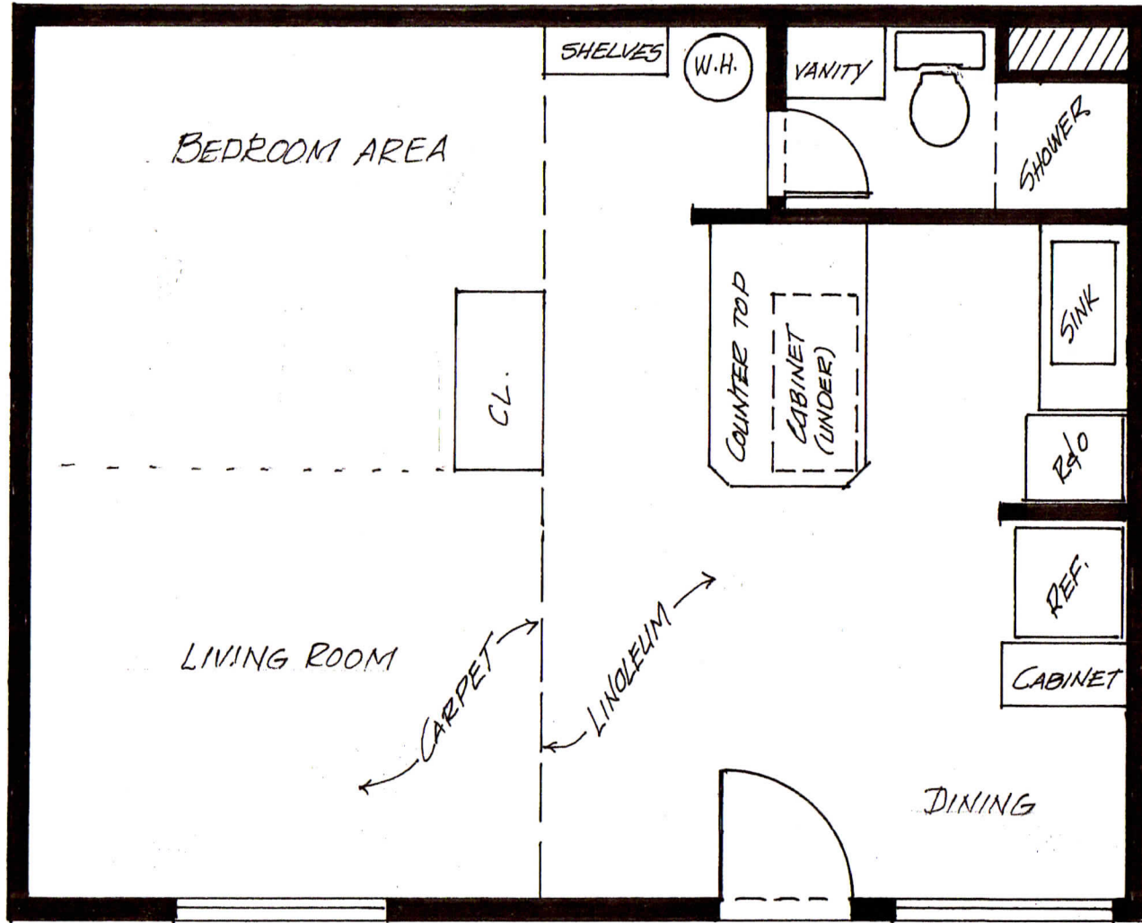
WESTSIDE LOFTS - TYPICAL 1-BEDROOM
