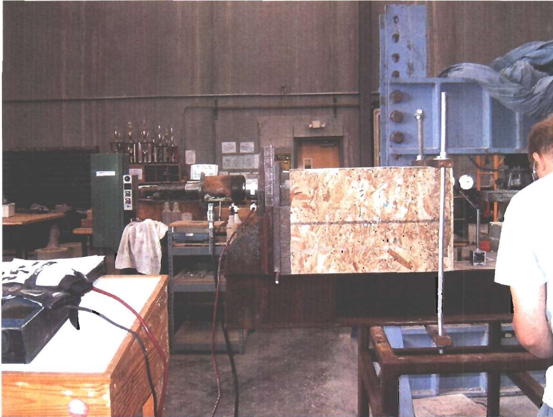
Photo 1: Test apparatus and specimen during testing
