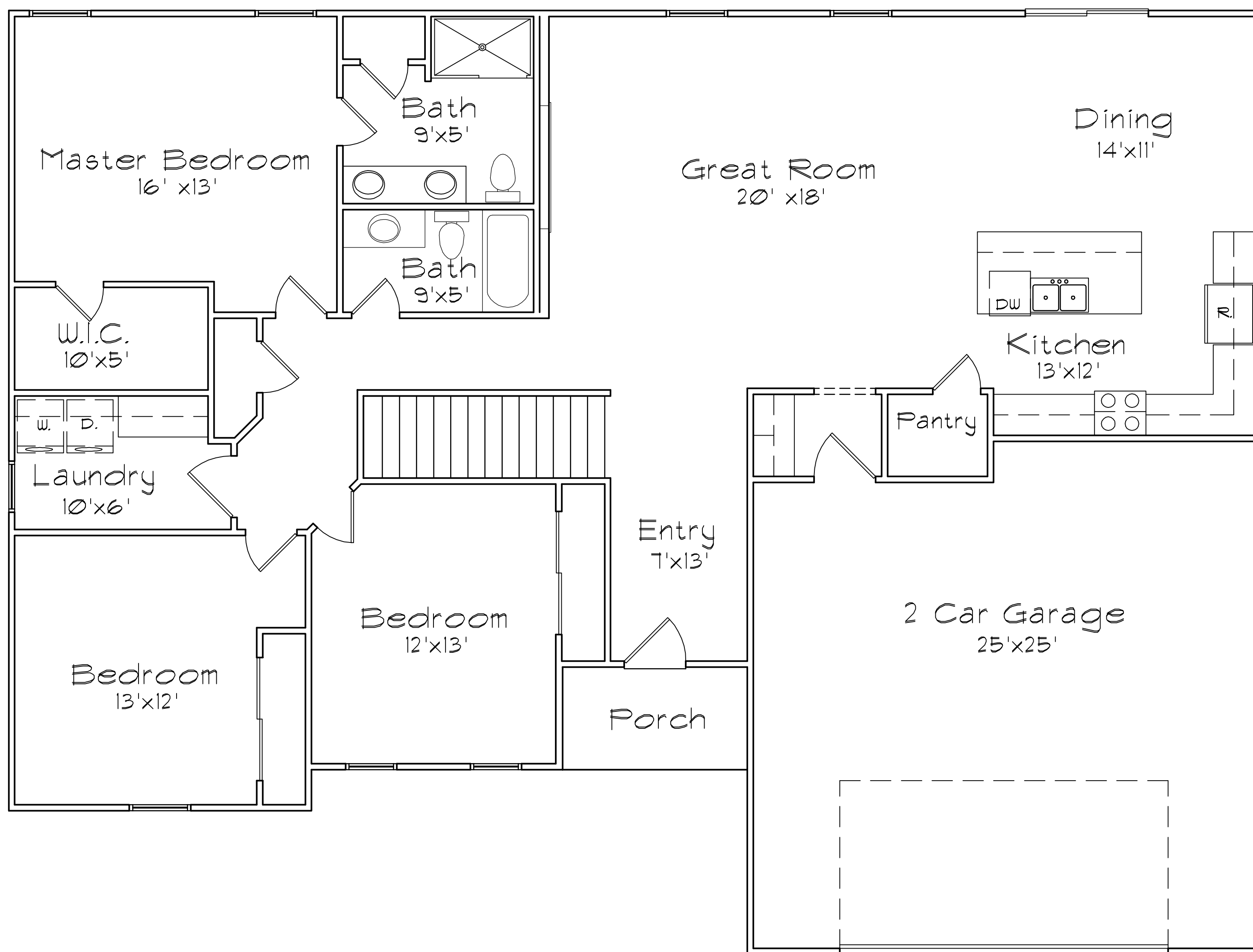
Floor Plan
