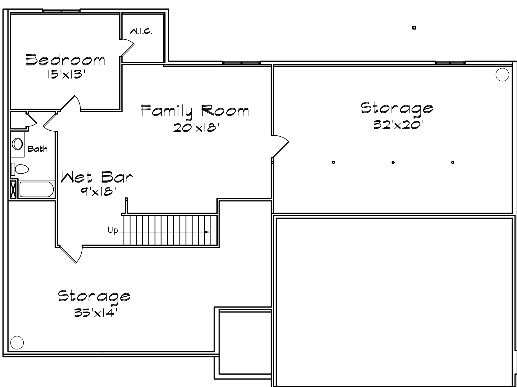
Basement Plan
