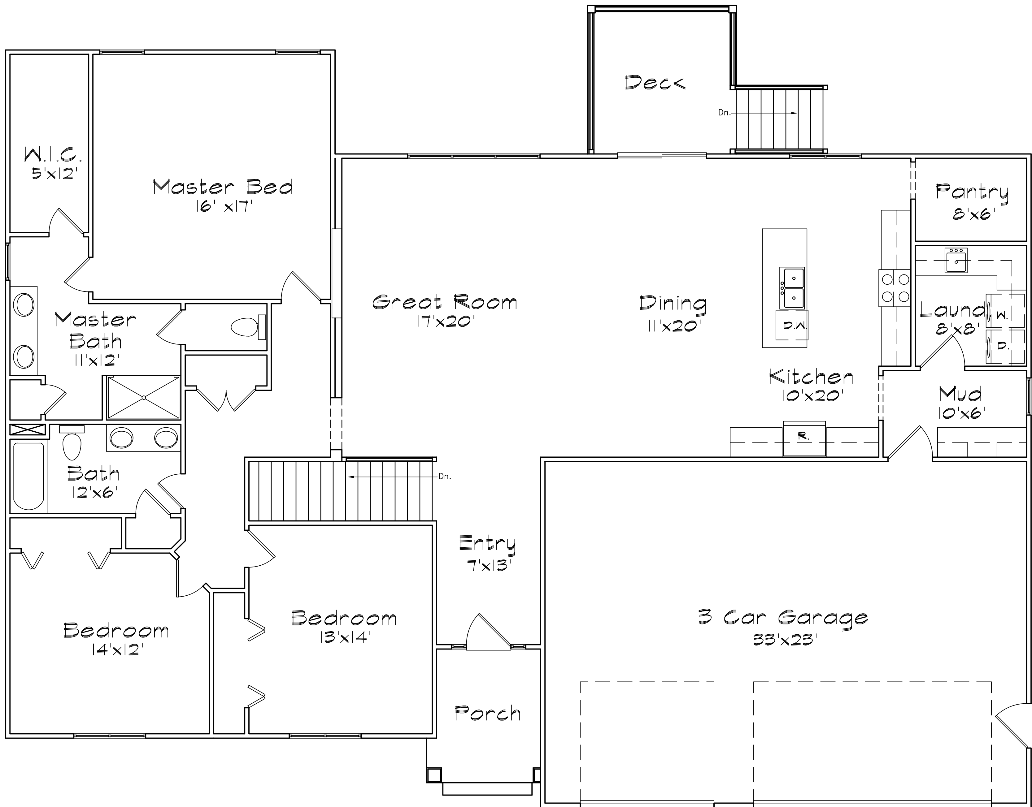
Floor Plan
