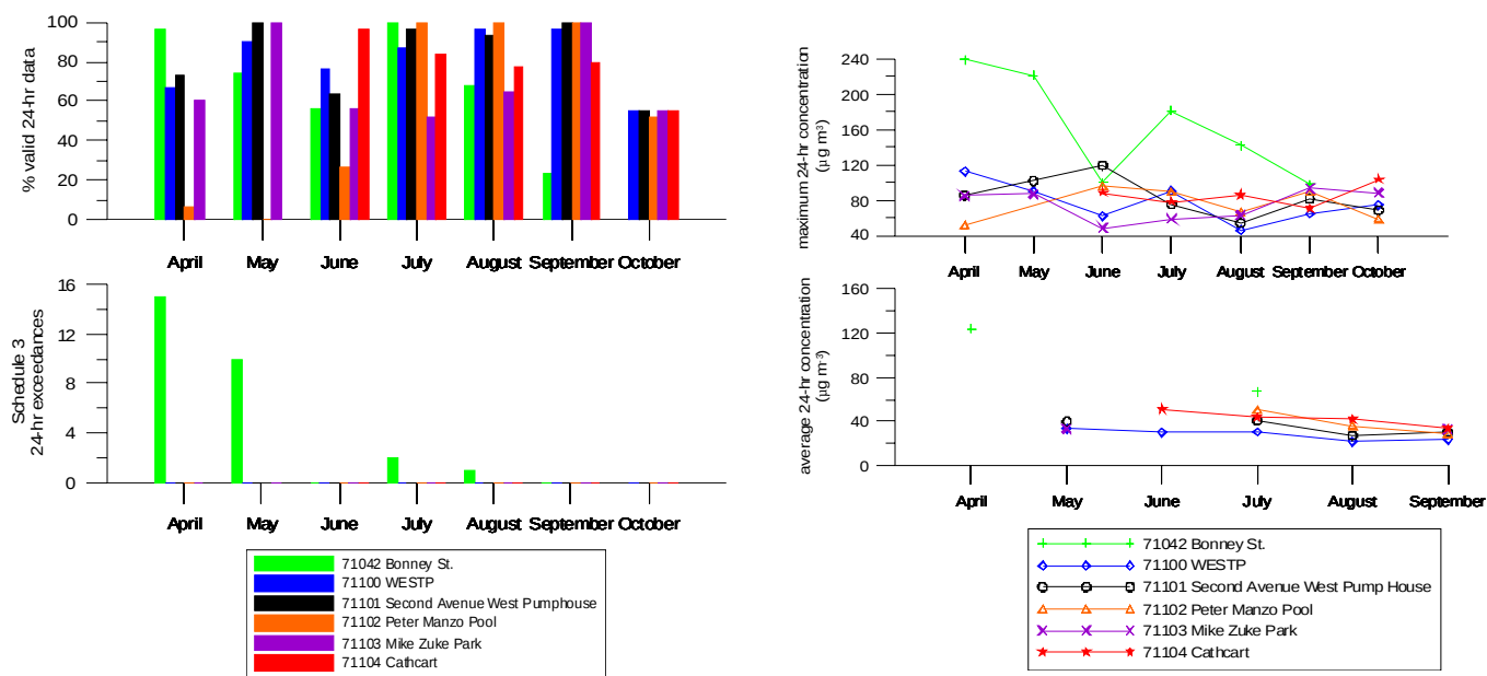
Figure 8: 24-hr TSP average statistics for the six monitoring locations presented by month
