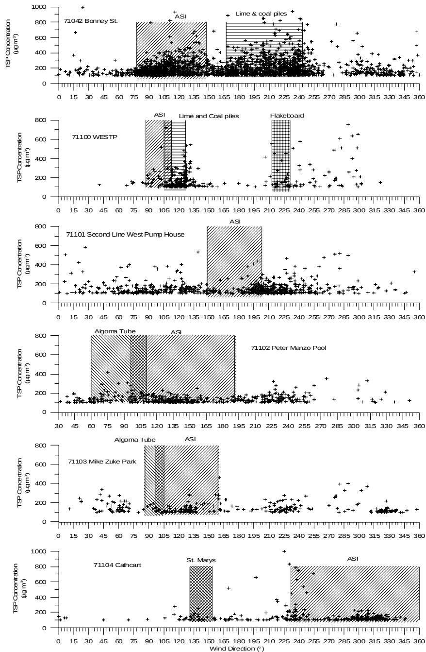
Figure 10: Wind direction analysis of 15 min average TSP data. Various industrial particulate sources are identified. Only TSP values greater than 100 \mu\text{g m}^{-3} have been included. Wind directions associated with wind speeds less than 3 \text{ km hr}^{-1} have been excluded since wind direction becomes unreliable at low wind speeds
