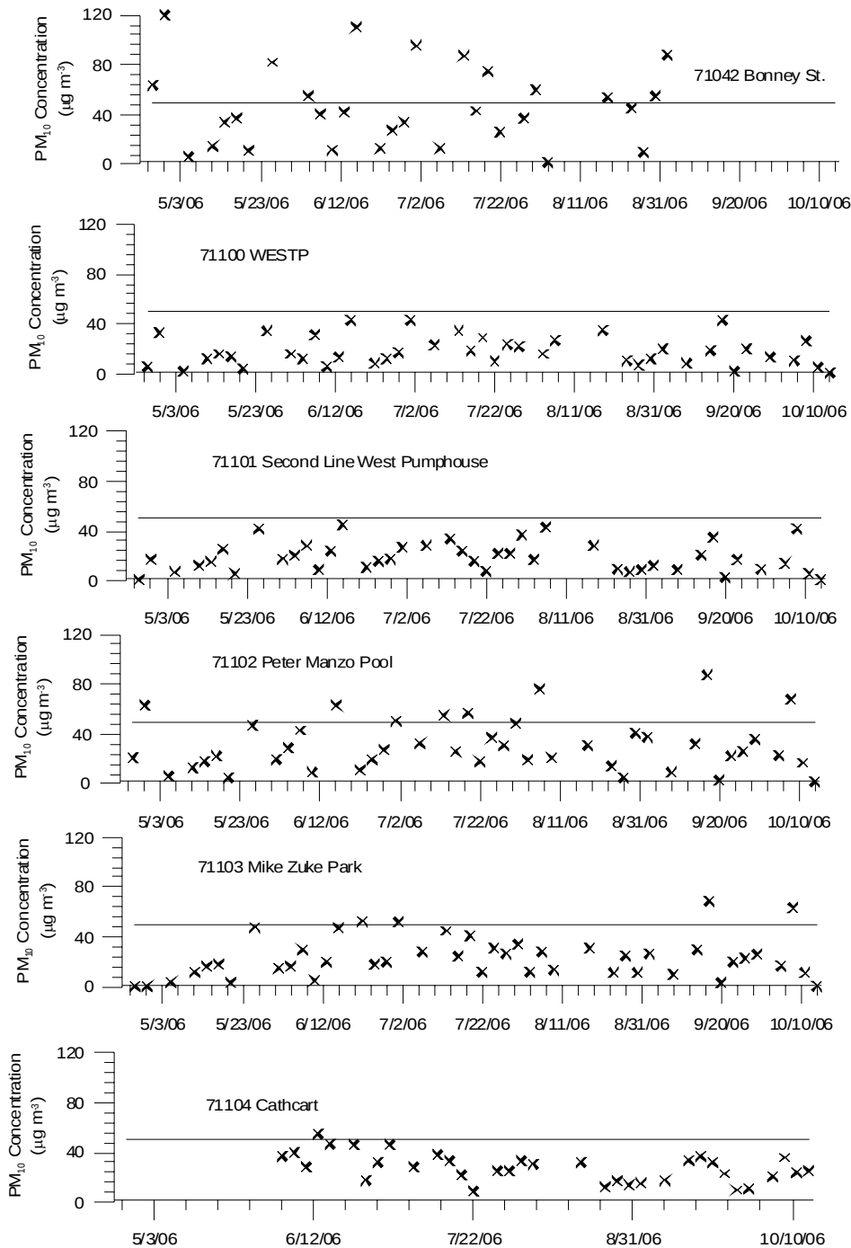
Figure 11: Time series presentation of PM 10 24-hr sampling results
