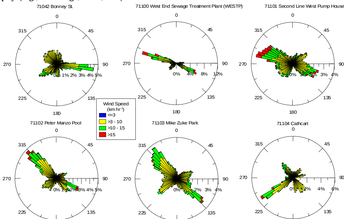
Figure 6: Wind roses for each of the 6 monitoring locations. Generated from the 15-min Aerocet data.
