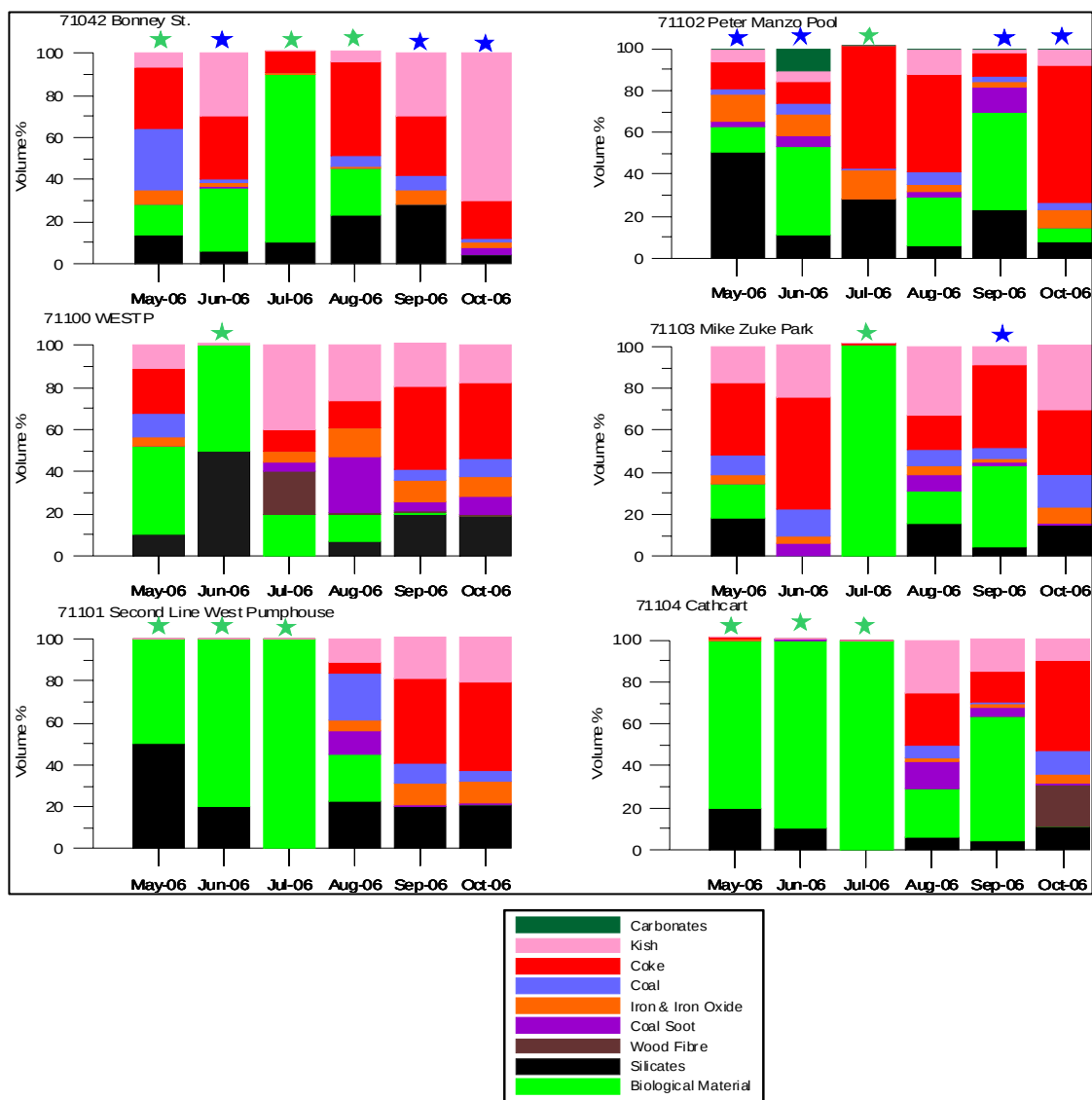
Figure 13: Optical characterisation results of dustfall samples collected at the 6 sampling locations. Blue stars identify exceedance samples. Green stars identify exceedance samples which contained algae.
