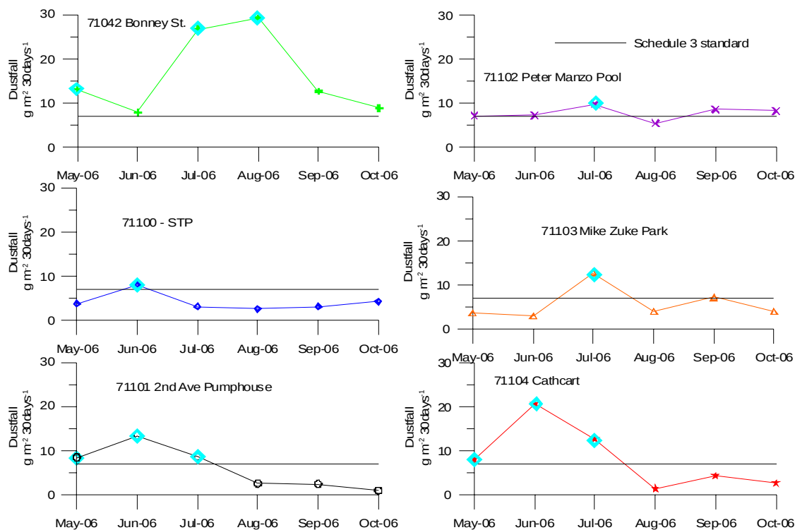
Figure 12: Summary of dustfall results May through October 2006 at the 6 sampling sites. The turquoise diamonds highlight samples in which algae was identified
