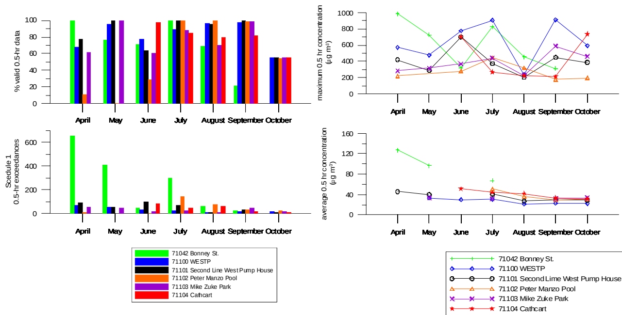
Figure 7: 0.5-hr TSP statistics for the 6 monitoring stations presented by month.
