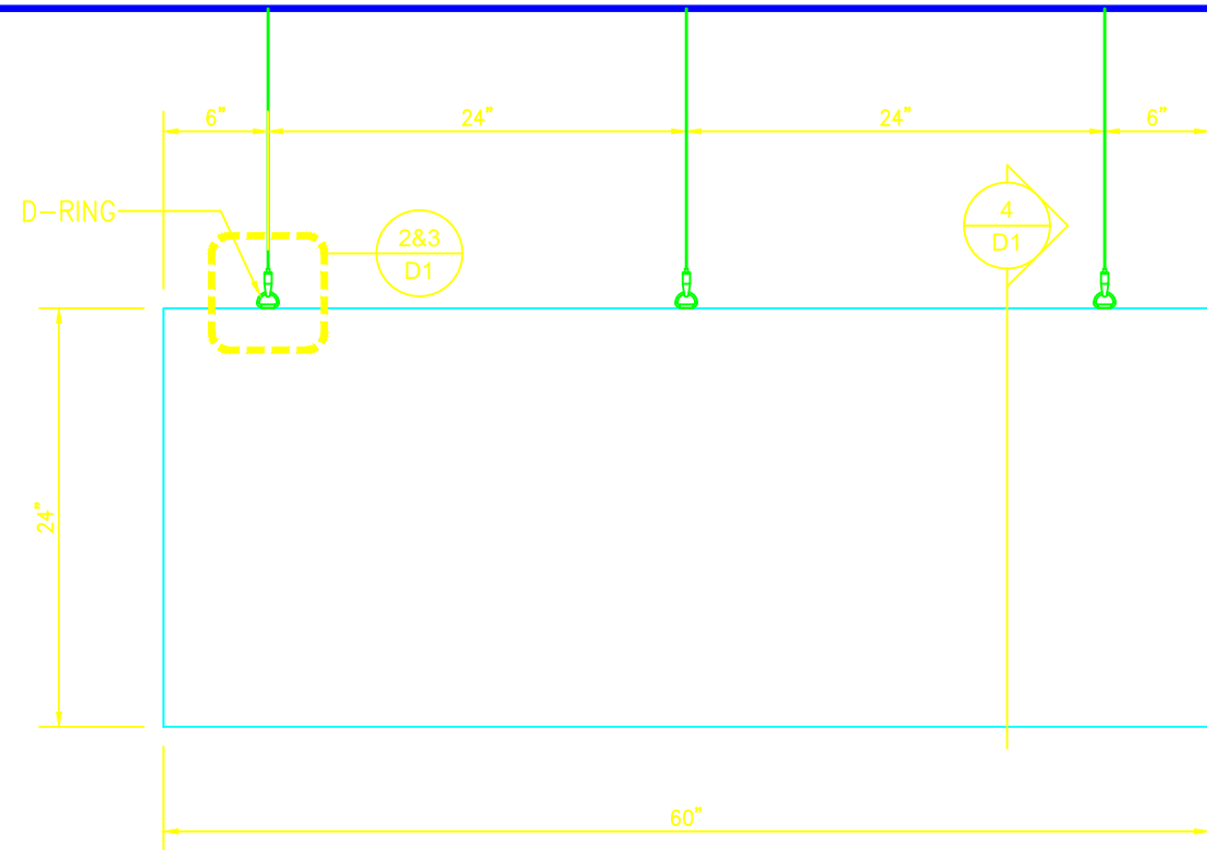
1 BAFFLE PANEL D1 SCALE 1"=1'-0"
