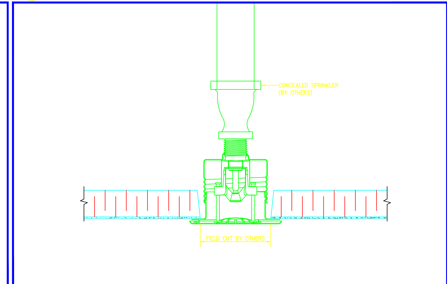
5 TYPICAL FIELD CUT DETAIL D1 SCALE 6"=1'-0"
