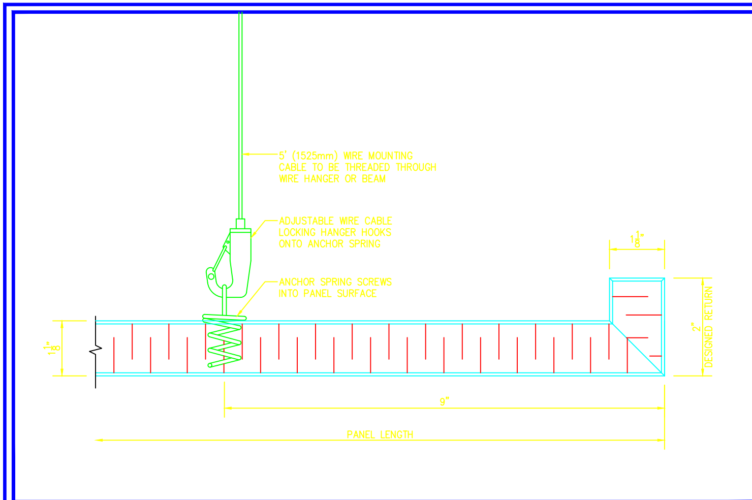
1 PERIMETER PANEL DETAIL D1 SCALE 6"=1'-0"
