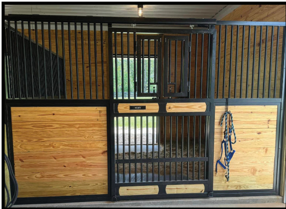
Legacy Stall Partition Located on the Left Side of the Stall & Dutch Door with Dutch Door Crib Rail Frame at the Back of the Stall
