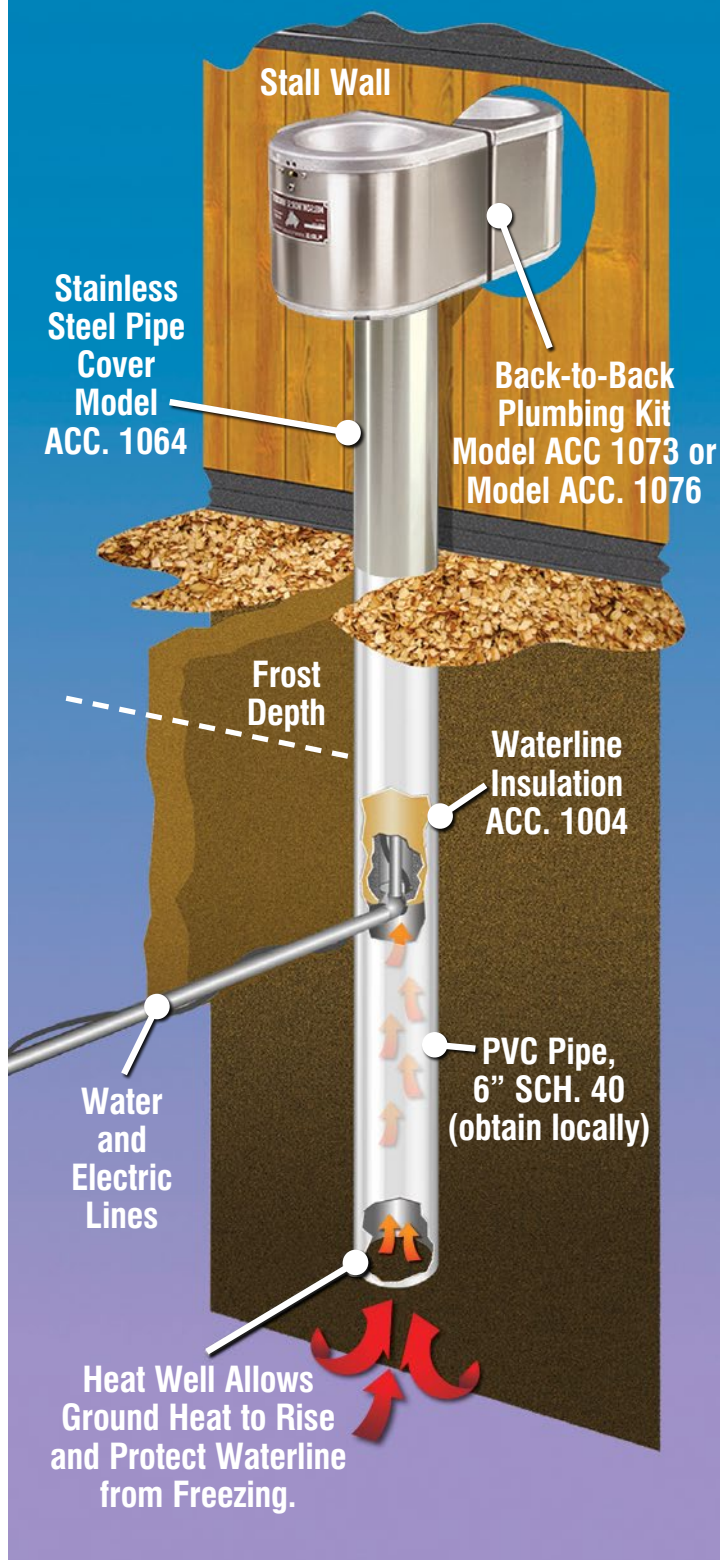
Model 730-10W or 760-10W
