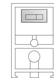
Dual Flush Concealed WC Cistern with Mid-Height Wall Hung Frame H820 - 880 x W515 max x D150 - 200mm XTY007 £394.00
