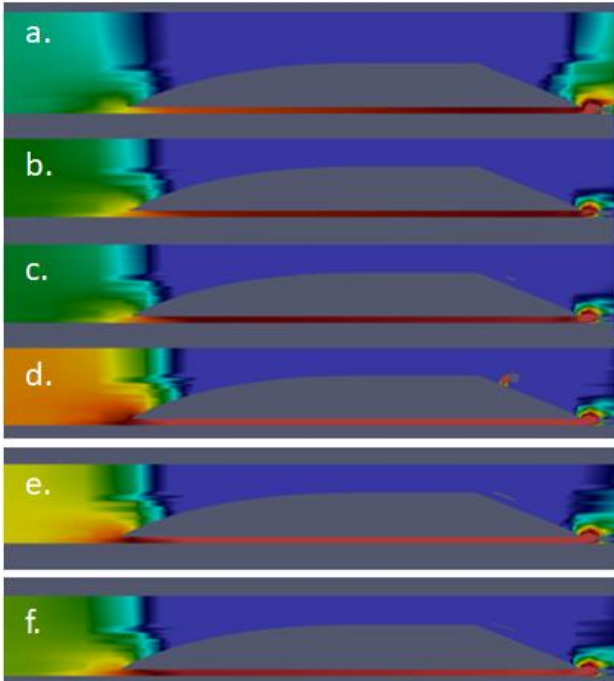
1 2 Figure 6. Pressure profiles of converged pressure profiles in tunnel with different upper 3 clearances and different versions of spoilers. 4
