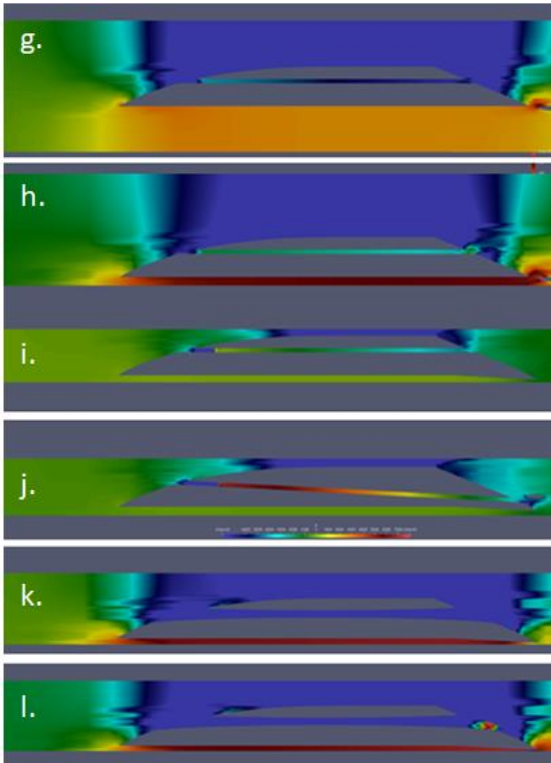
1 2 Figure 7. Pressure profiles of converged pressure profiles in tunnel with different 3 clearances and front-to-back bypass duct with bypass Sources. 4 5
