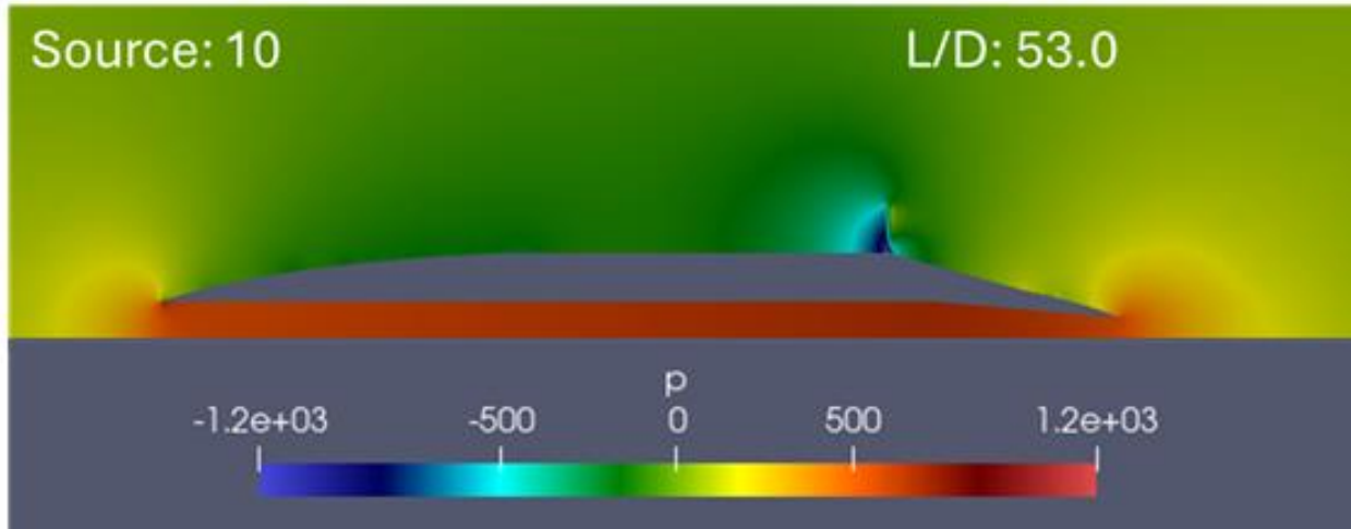
1 Figure 1. Example of a high L/D benchmark pressure profile. A cross section of a 2 3D prototype simulation using fences to block losses of lower compartment lift 3 pressures. Free stream velocity is 40 m/s and the Source is in \text{m}^4/\text{s}^2 . 4 5
