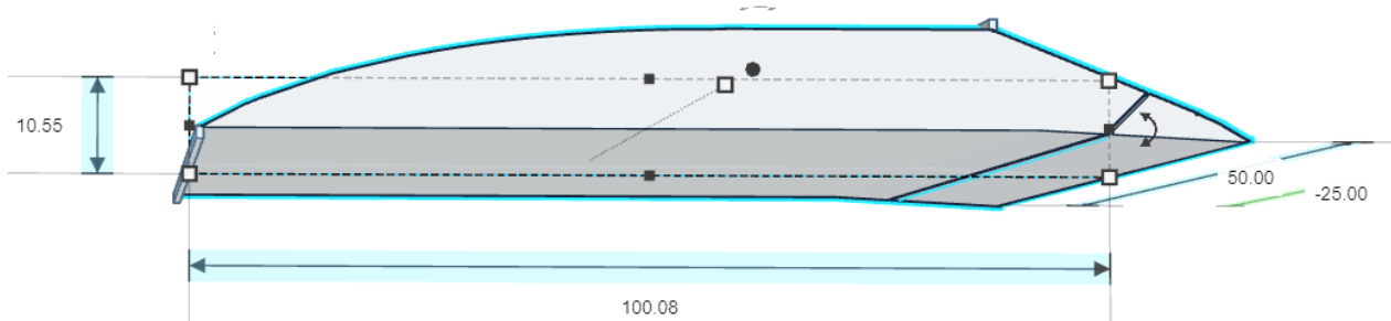
1 Figure 3. Illustration of computer-aided design (CAD) STL file (standard template 2 library) of lifting body with upper and lower sources and a trailing section bypass from 3 the cavity (height = 0.01 m) to the upper surface of the trailing taper. Dimensions are in 4 cm. 5 6
