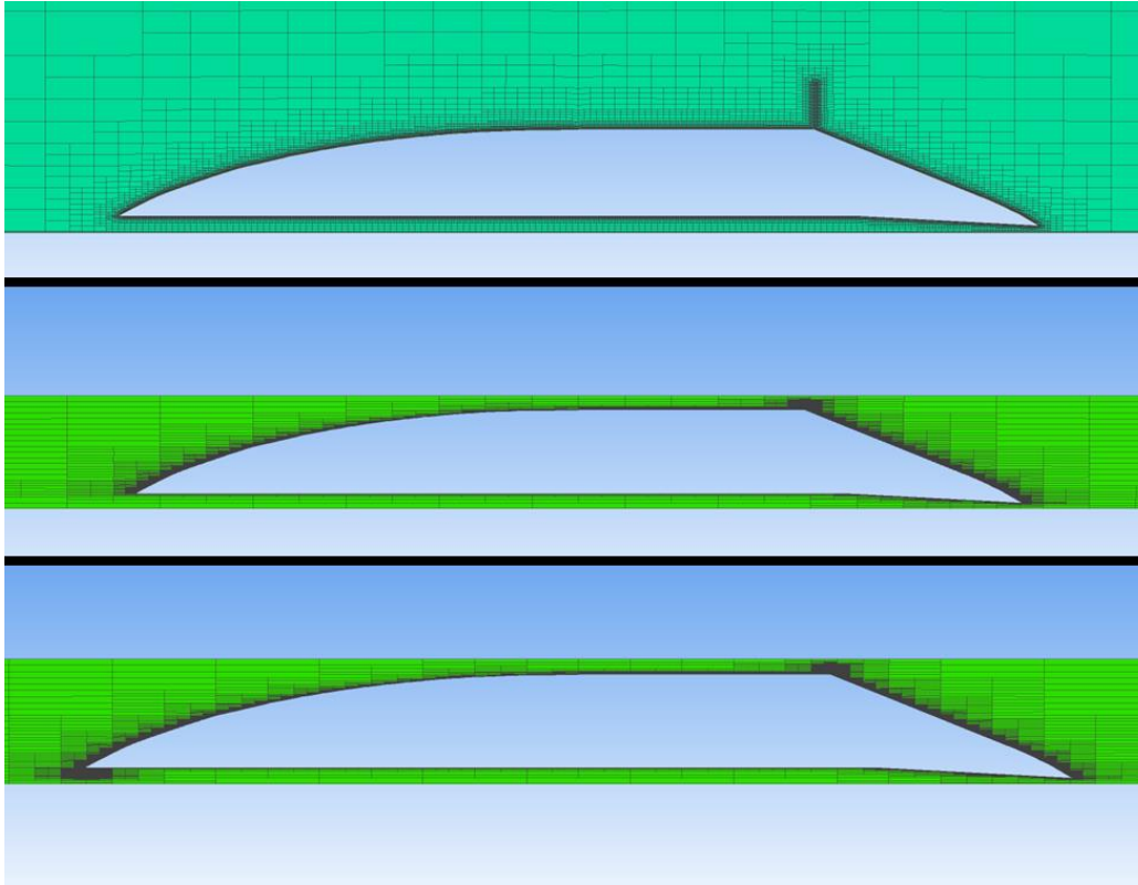
6 7 Figure 2. CFD meshes for 0.1 t/c airfoil of 1 m length with one upper Source 8 0.05X0.005 m Source (upper) with 0.004 m clearance to ground, one upper Sources in 9 tunnel of 0.004 m upper and lower clearances (middle), and upper and lower sources of 10 0.01X0.005 m Sources. Cavity height is 0.01 m.
