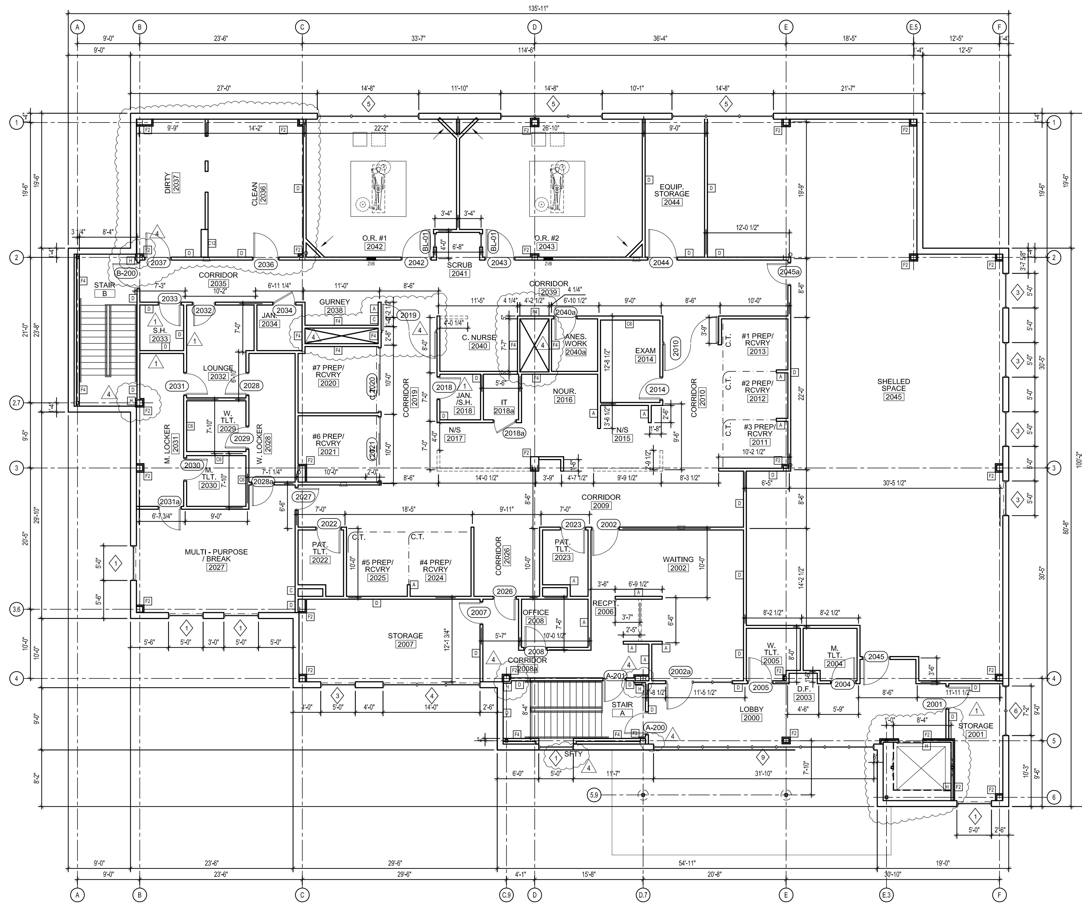
1 SECOND FLOOR - DIMENSION PLAN SCALE: 1/8" = 1'-0"
