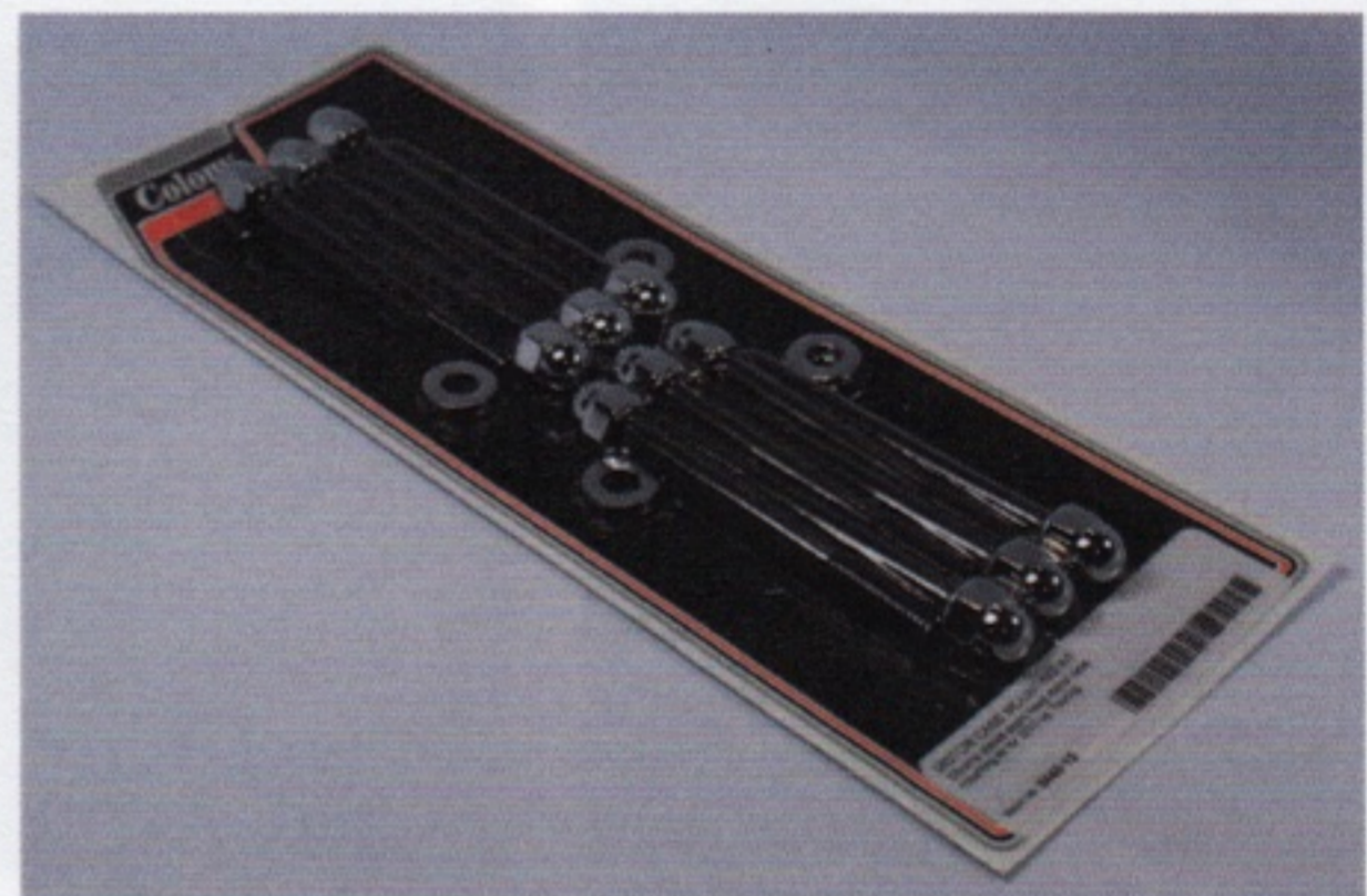
Part No. 3440-12 MOTOR CASE MOUNTING KIT Chrome plated acorn head motor case mounting kit for 2017-up Touring. Retail: $40.92 Dealer: $26.59
