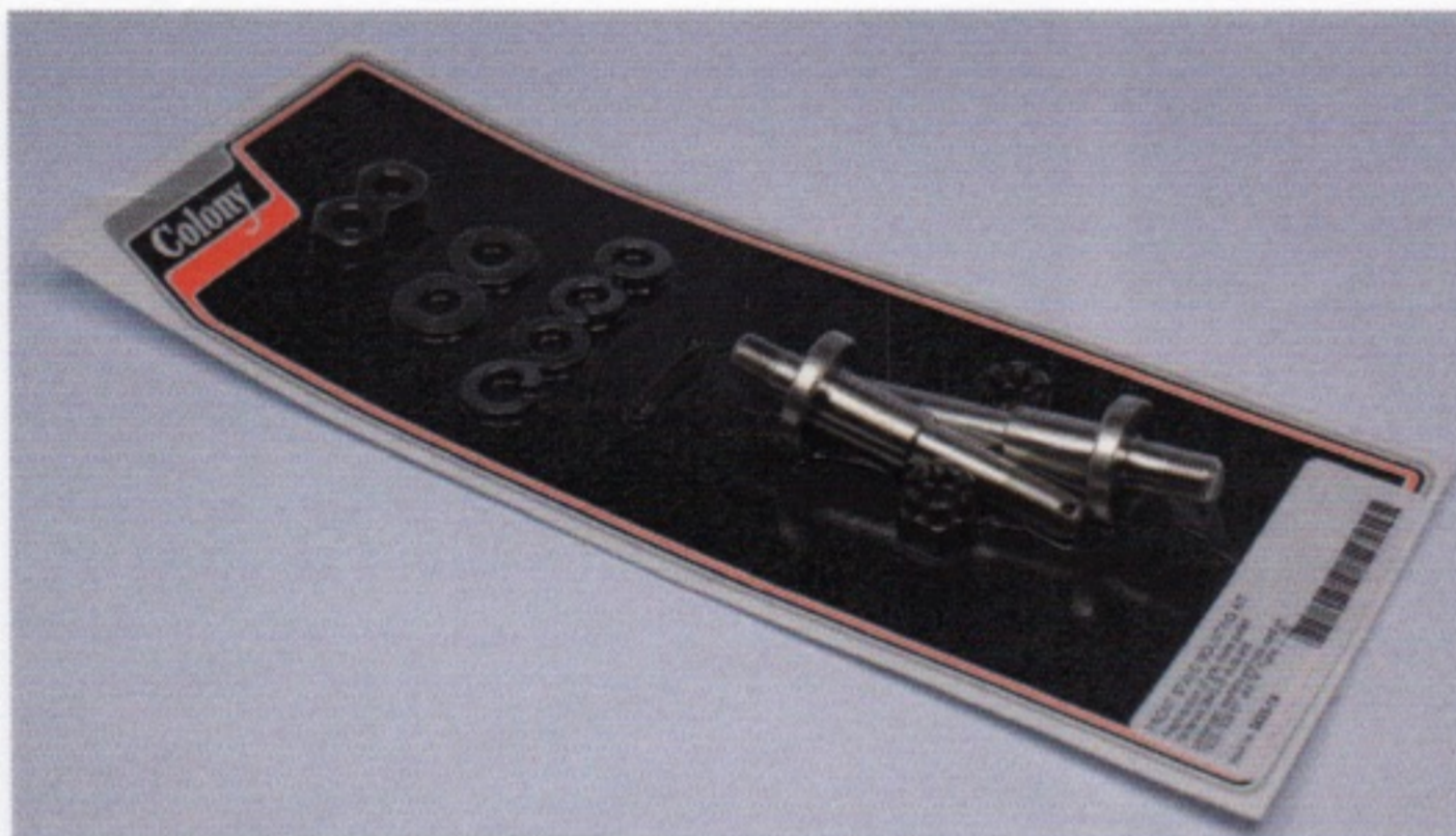
Part No. 3433-14 FRONT STAND MOUNTING KIT Reproduction of gray nickle plated hardened 2640-25 studs and parkerized washers and nuts used on 1925-1929 61 and 74" Twins. J, JD. Retail: $38.25
