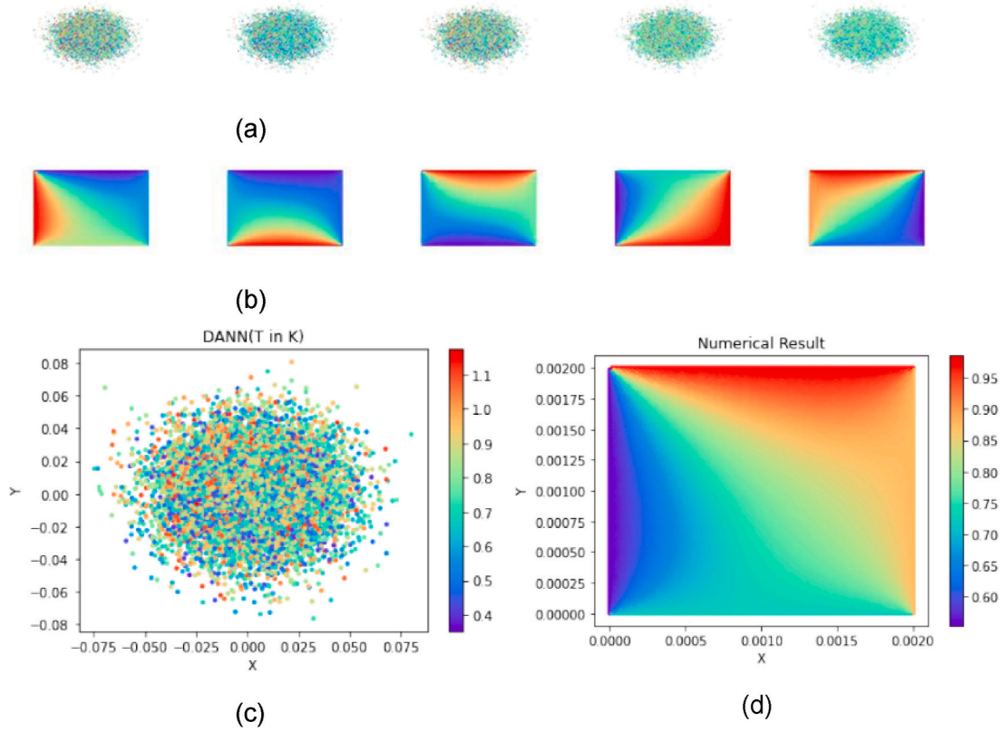
Fig. 8. DL based DANN model to predict heat conduction.
