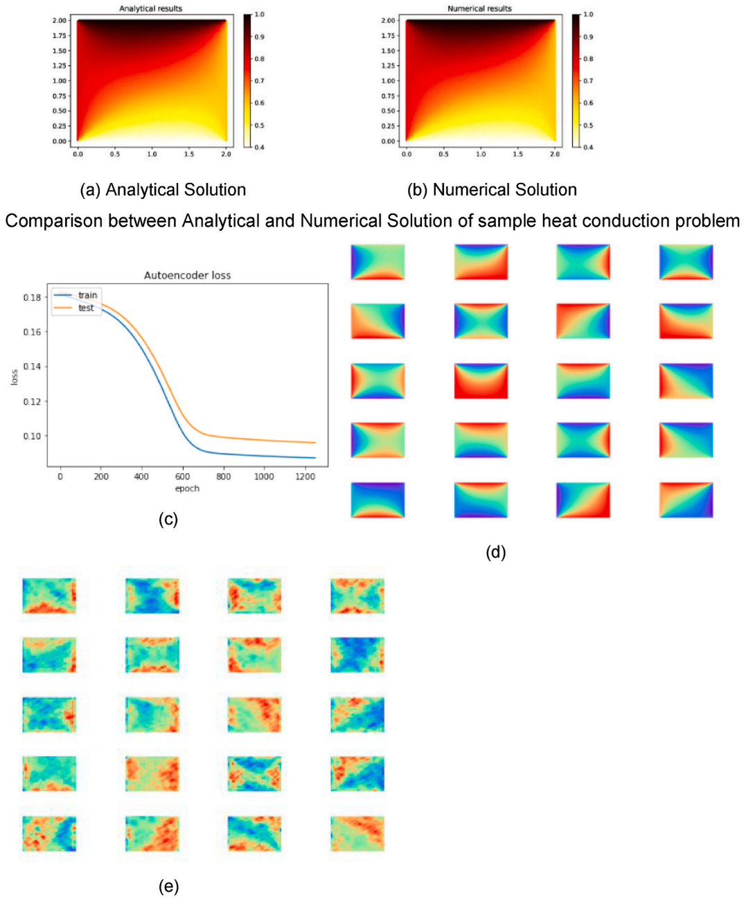
Fig. 6. DL based Autoencoder model to predict heat conduction.
