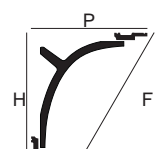
C991 + 2x P9900 LUXXUS
