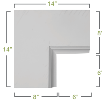
PERIMETER INSIDE CORNER
