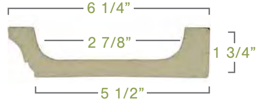
PERIMETER BEAM
