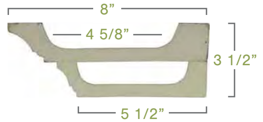
PERIMETER BEAM
