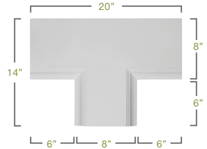
PERIMETER TEE
