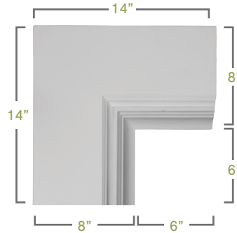
PERIMETER INSIDE CORNER
