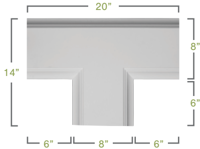
INNER TEE
