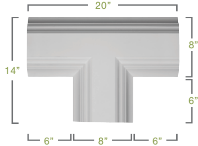
INNER TEE
