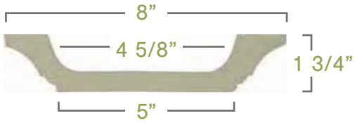
INNER BEAM
