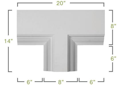
PERIMETER TEE
