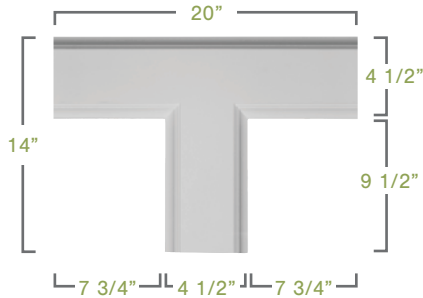
INNER TEE
