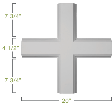
INNER CROSS INTERSECTION
