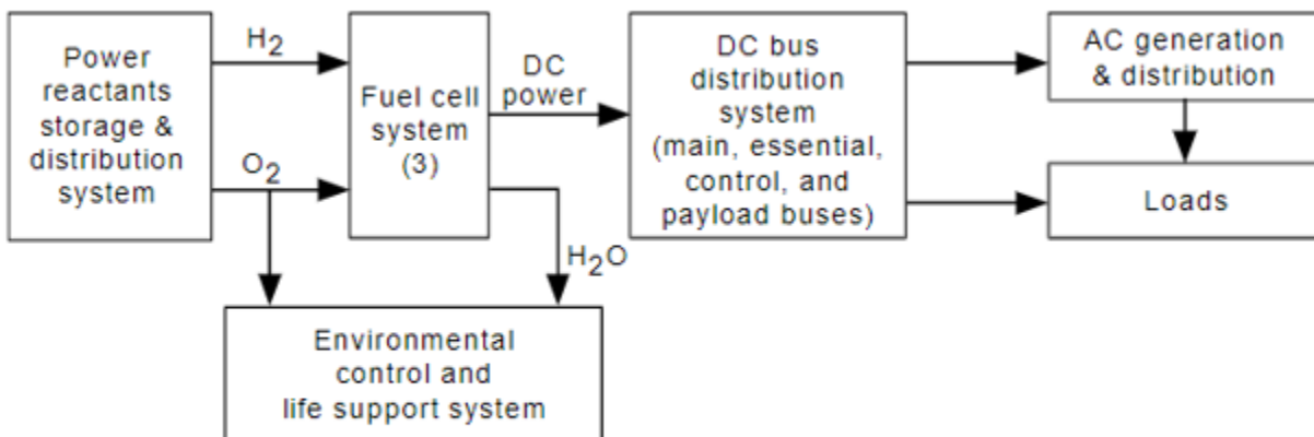
The Electrical Power System
