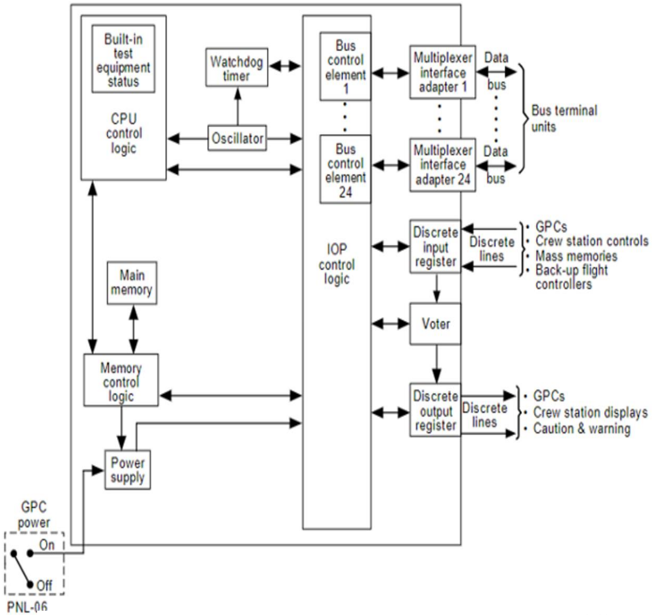
GENERAL PURPOSE COMPUTER FUNCTIONAL BLOCK DIAGRAM
