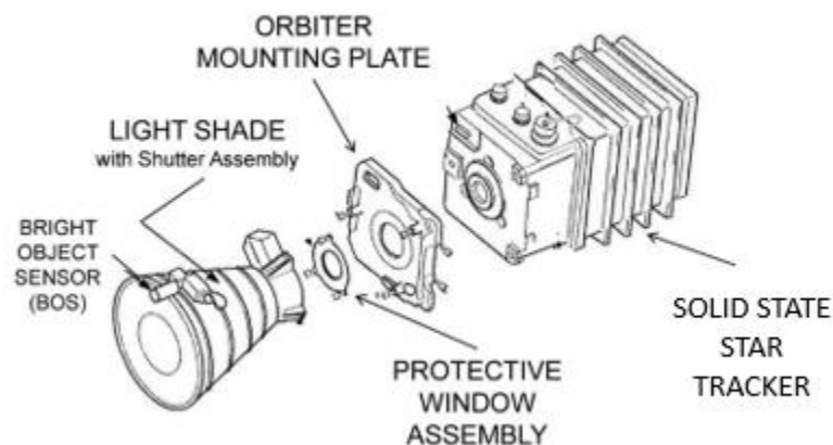
STAR TRACKER
