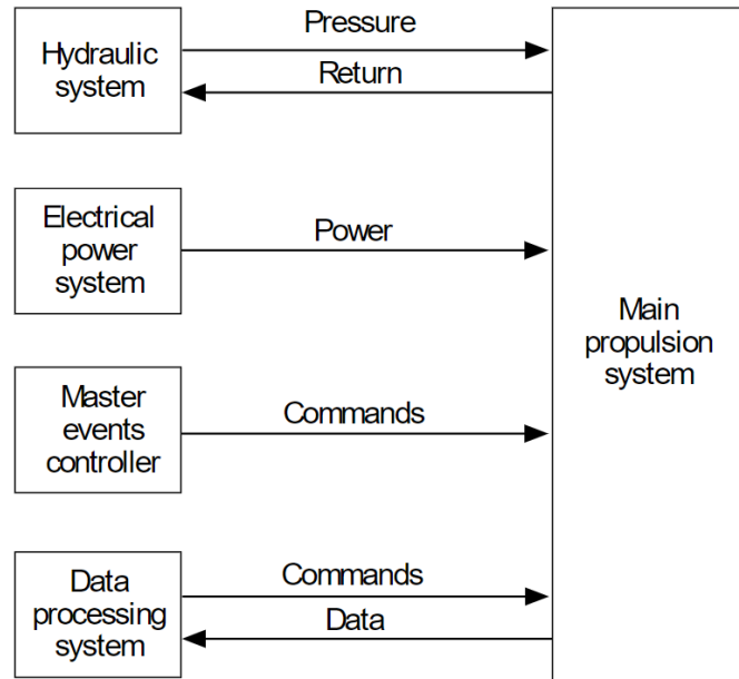
CRITICAL INTERFACES WITH THE MAIN PROPULSION SYSTEM
