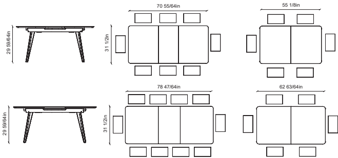
Kitchen table MODENA DT-MODENA 55(70)x31x29 Laminam Bianco Statuario Venato DT-MODENA 62(78)x31x29 Laminam Bianco Statuario Venato Tabletop Material: Top – Ceramic Italy (5 mm), bottom – MDF 19 mm. MDF Color Black Stain Base Material: Metal with powder coating technology (Mikroton paint, black) Opening Method: Side
