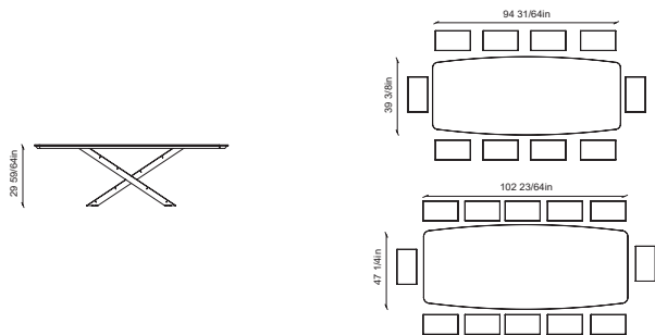
Kitchen table "COMO" DT-COMO 102x47x29 Laminam Bianco Statuario Venato Tabletop material: Triple glass: top ceramic 5 mm + bottom glass 4 mm (non-tempered) / wooden base 35 mm, angled at 45° Base material: metal with powder coating technology (Mikroton paint, black)
