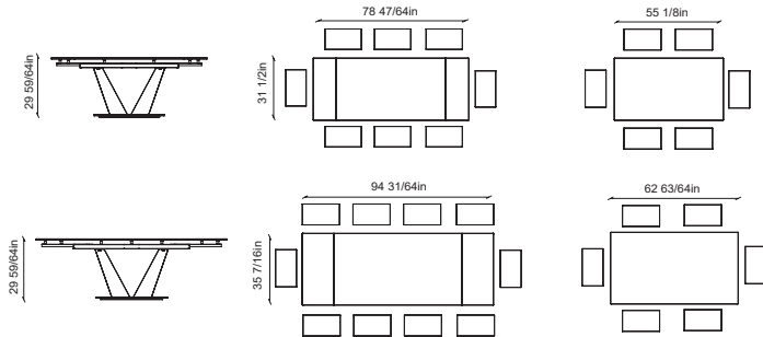
Kitchen Table "PARMA" Model: DT-PARMA 55(78)x31x29 Laminam Bianco Statuario Venato Model: DT-PARMA 62(94)x35x29 Laminam Bianco Statuario Venato Tabletop Material: Italian triple-layered ceramic 3 mm + tempered glass Saint-Gobain 8 mm Base Material: Metal with powder coating technology (Mikroton paint, black) Opening Mechanism: Side
