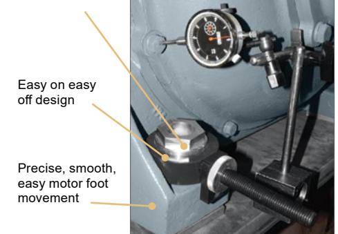
Eccentric socket
