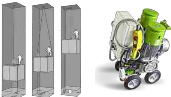
Dual Lift Hoist for Elevator Installation & Maintenance
