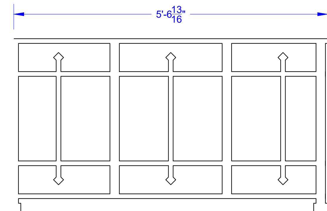
6.4 POLICE PLATFORM RAILING SCALE: 1" = 1' - 0"
