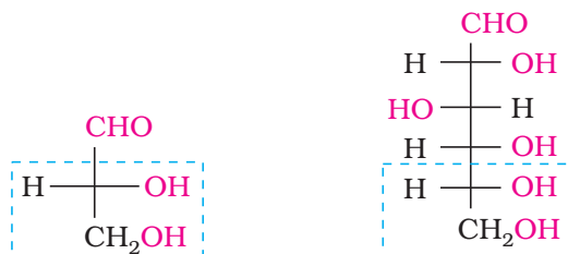
D- (+) - Glyceraldehyde
