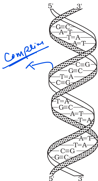
Fig. 14.7: Double strand helix structure for DNA
