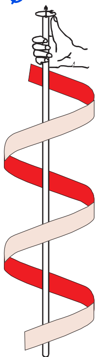
Fig. 14.1: \alpha -Helix structure of proteins
