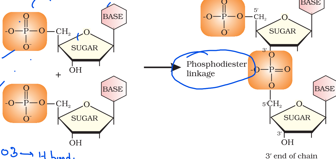
Fig. 14.6: Formation of a dinucleotide
