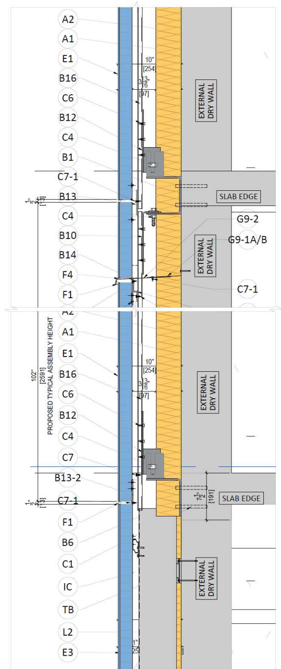
1 SECTION DETAIL-01 MT-404 SCALE: 1-1/2"=1'
