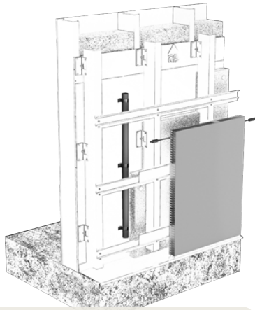
• CladiShield System (Rainscreen System)
