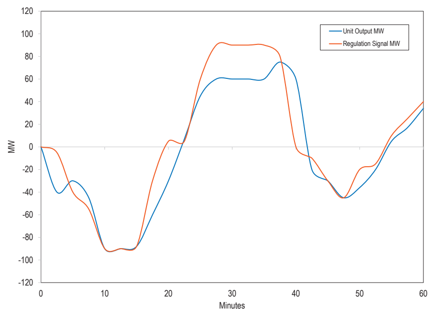
Figure 10-31 A unit providing 100 MW of regulation while following an almost neutral regulation signal
