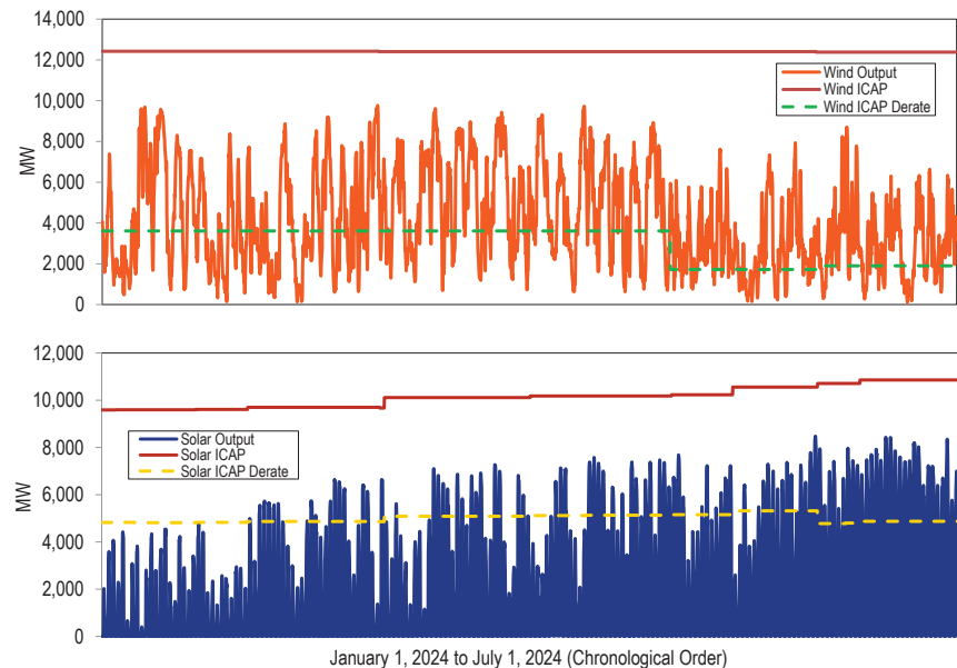
Figure 8-15 Wind and solar output: January through June, 2024
