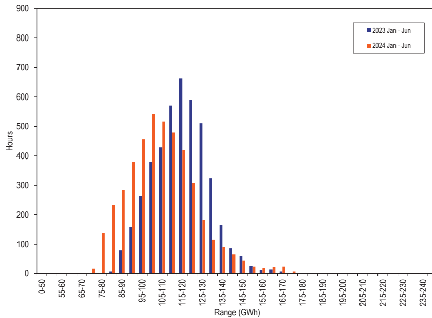
Figure 3-13 Distribution of day-ahead cleared demand plus exports: January through June, 2023 and 2024 39
