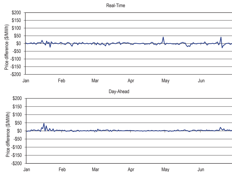
Figure 9-6 Price differences (NY/PJM proxy - PJM/NYIS Interface): January through June, 2024
