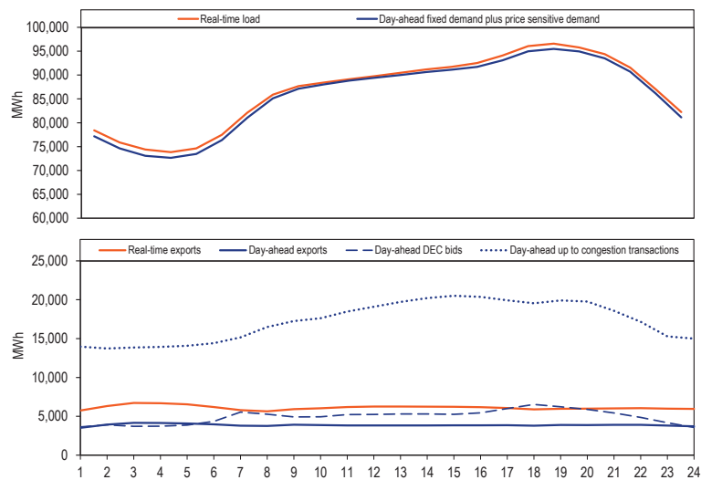
Figure 3-15 Day-ahead and real-time demand (Average hourly volumes): January through June, 2024
