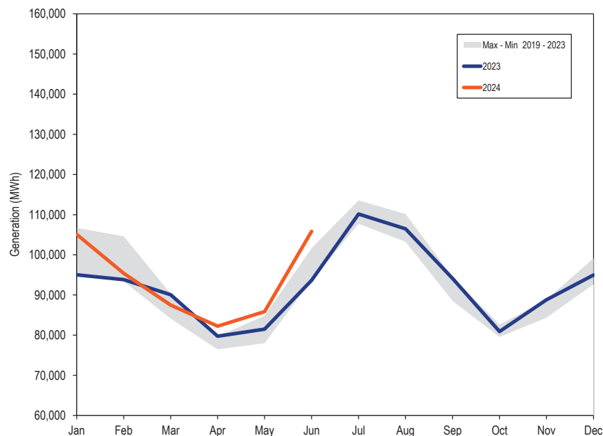
Figure 3-4 Real-time monthly average generation: 2023 through June 2024
