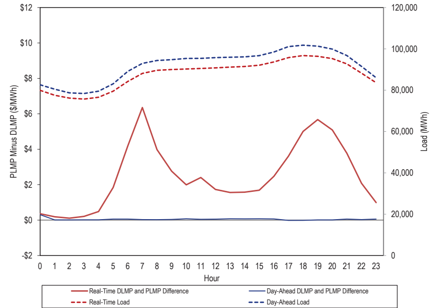
Figure 3-27 Hourly average load and LMP difference: January through June, 2024
