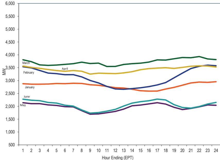
Figure 8-17 Average hourly day-ahead generation of wind units: January through June, 2024
