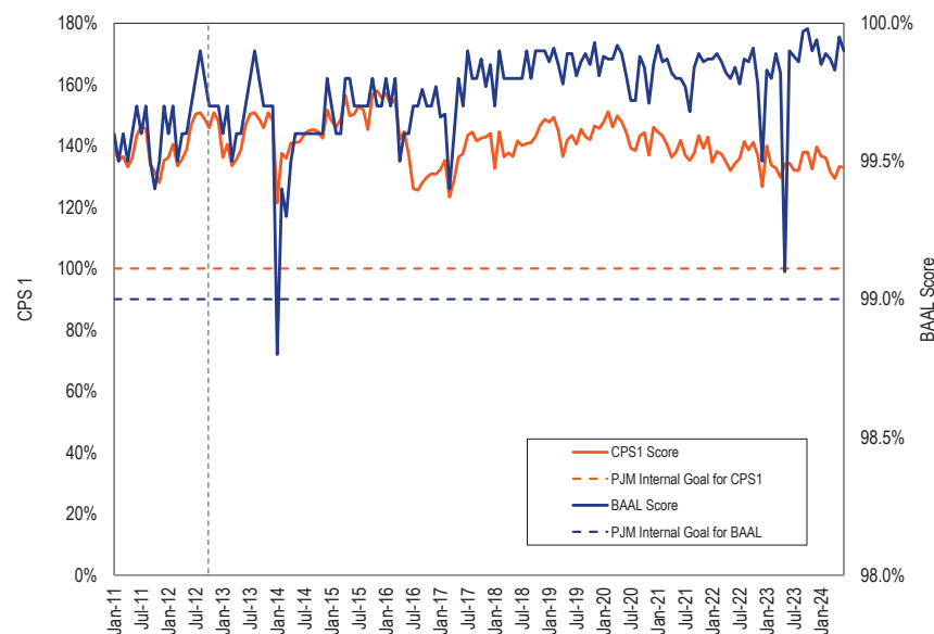
Figure 10-41 Monthly CPS1 and BAAL performance: January 2011 through June 2024
