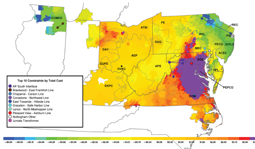
Figure 11-7 Location of the top 10 constraints by total congestion costs: January through June, 2024
