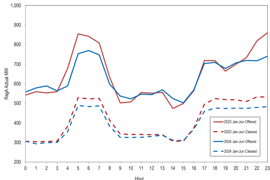
Figure 10-37 Average hourly RegA actual MW offered and cleared: January through June, 2023 through 2024 103
