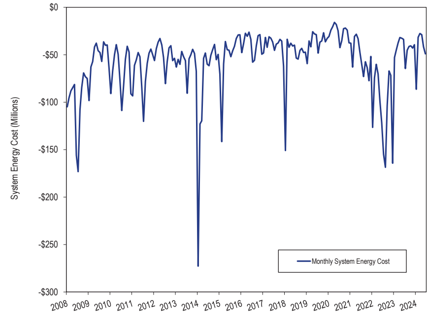
Figure 11-12 Monthly system energy costs (Millions): January 2008 through June 2024
