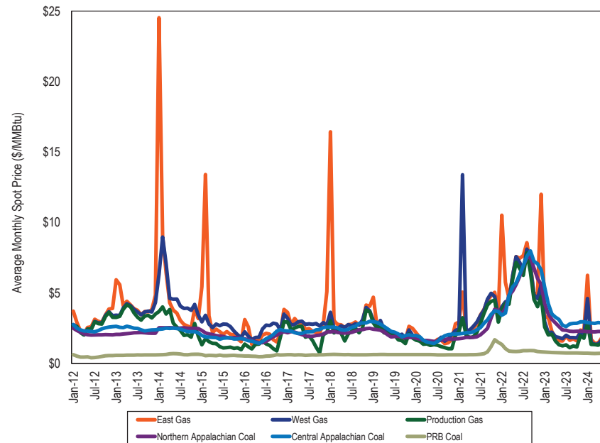
Figure 3-49 Spot average fuel price comparison: 2012 through June 2024 ($/MMBtu)
