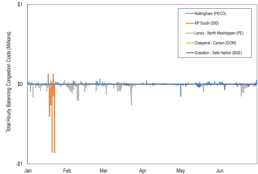
Figure 11-5 Top five constraints affecting balancing congestion costs: January through June, 2024
