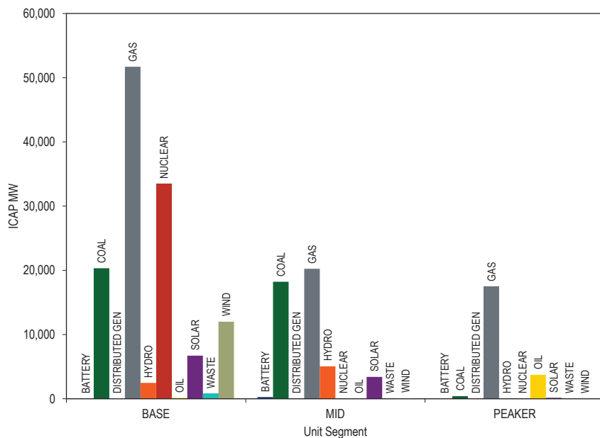
Figure 3-53 Real-time ICAP distribution by fuel and segment: January through June, 2024 142
