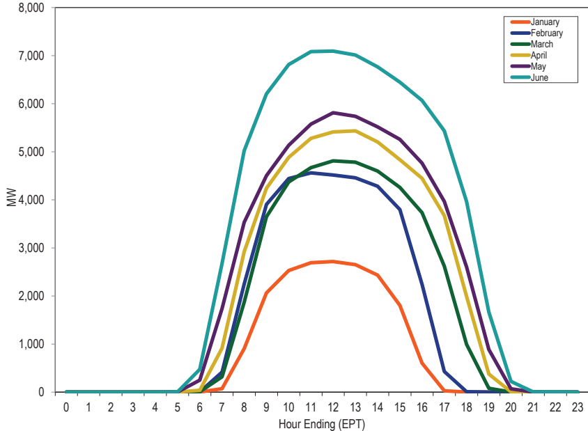
Figure 8-19 Average hourly real-time generation of solar units: January through June, 2024
