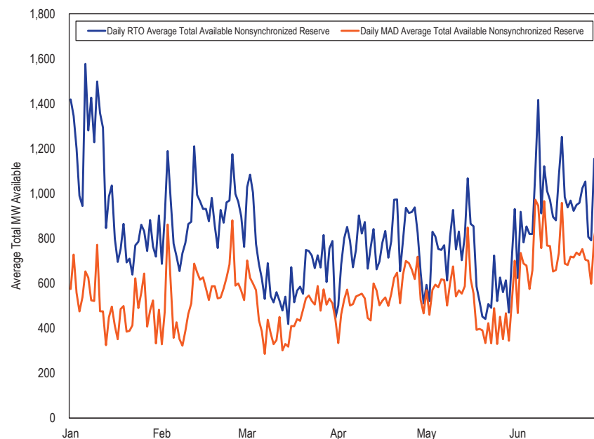
Figure 10-23 Daily Average Available Nonsynchronized Reserve: January through June, 2024
