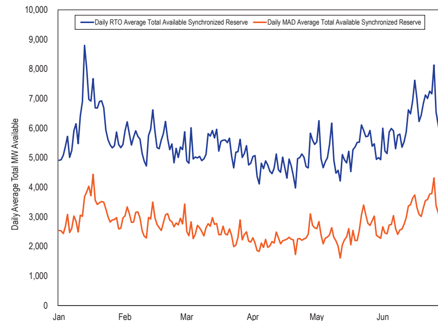
Figure 10-10 Daily Average Available Synchronized Reserve: January through June, 2024
