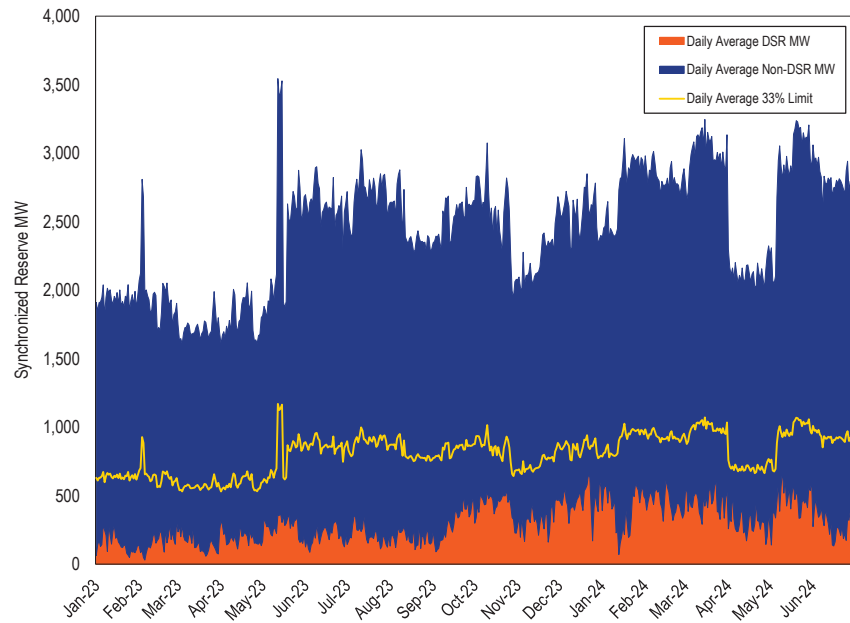
Figure 10-14 Daily average synchronized reserve from DSR and non-DSR: January 2023 through June 2024
