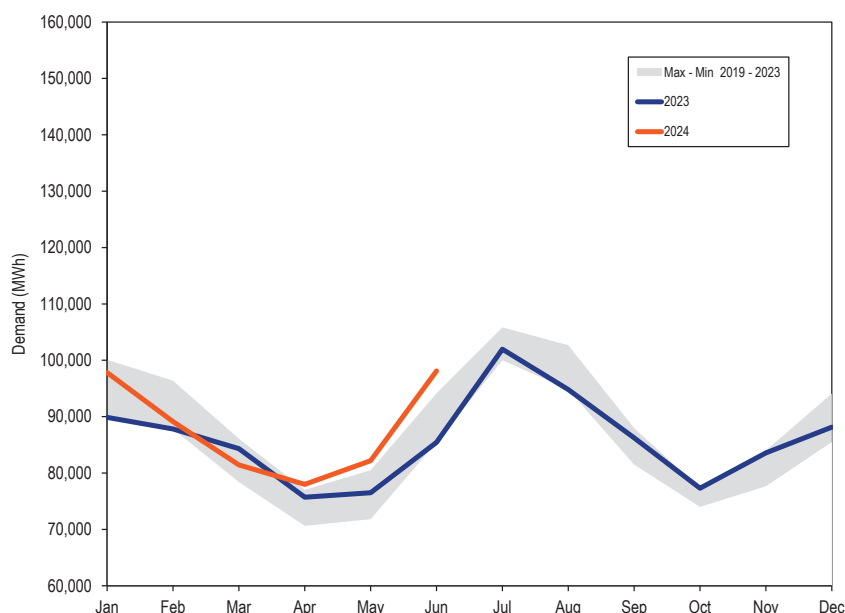
Figure 3-11 Real-time monthly average hourly load plus exports: 2023 through June 2024
