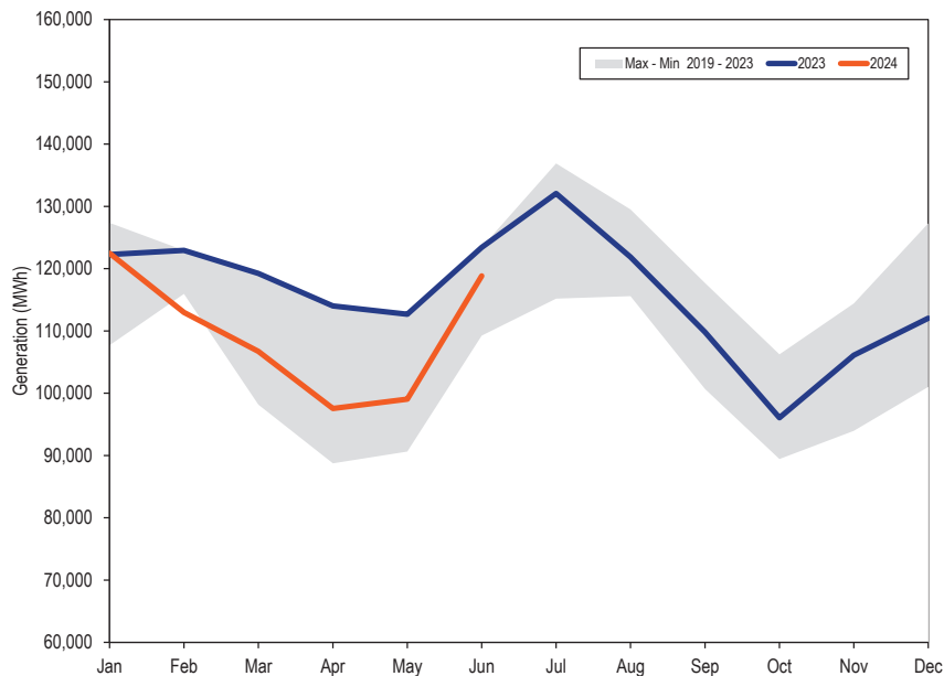
Figure 3-6 Day-ahead monthly average cleared supply: 2023 through June 2024
