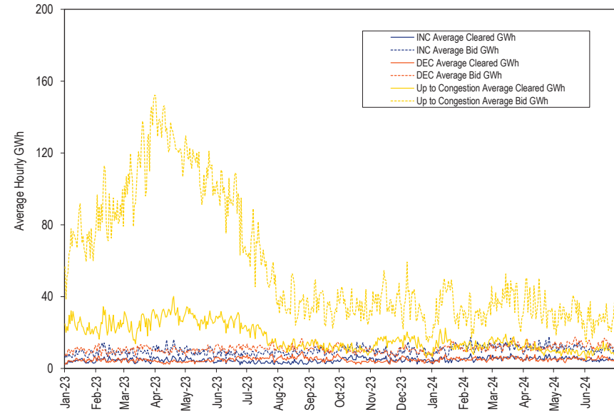
Figure 3-22 Daily bid and cleared INCs, DECs, and UTCs (GWh): January 2023 through June 2024
