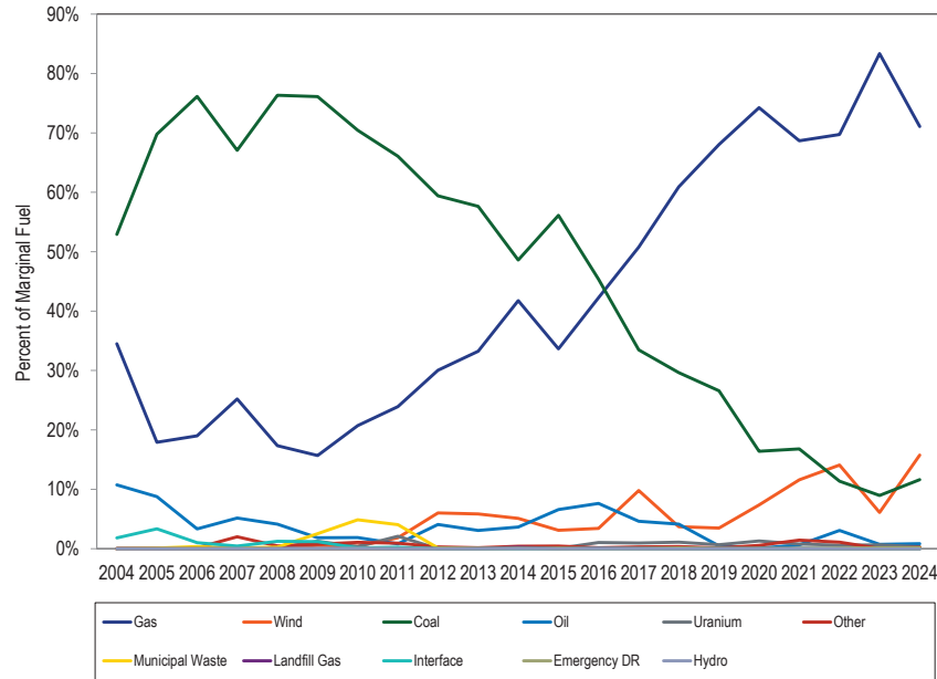
Figure 3-48 Type of fuel used (By real-time marginal units): January through June, 2004 through 2024
