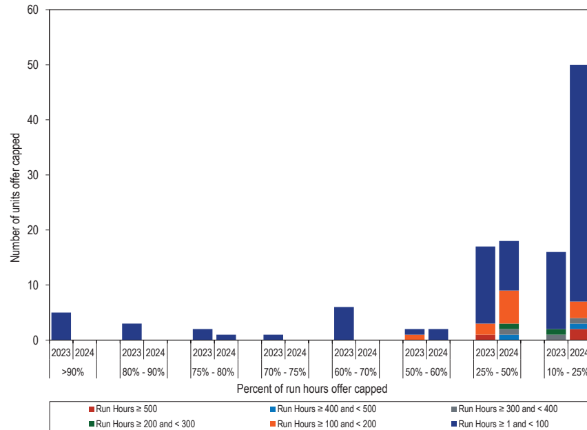
Figure 3-60 Real-time offer capped unit statistics: January through June, 2023 and 2024
