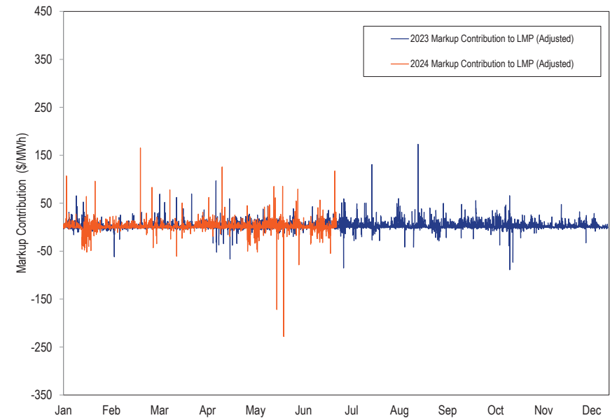
Figure 3-67 Markup contribution to real-time hourly load-weighted LMP (Adjusted): January 2023 through June 2024
