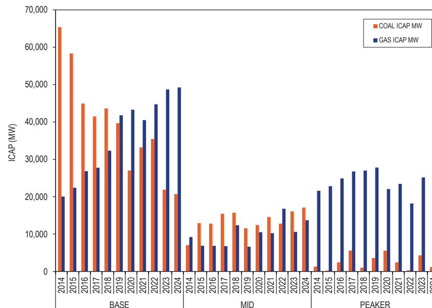
Figure 3-54 Real-time annual gas and coal unit segment classification: January through June, 2014 through 2024
