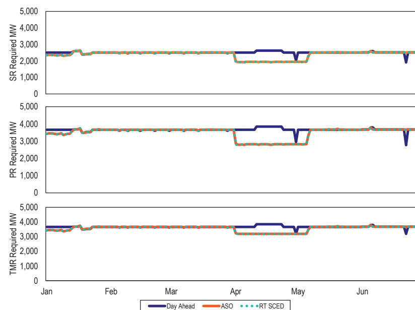
Figure 10-4 Requirements used in the day-ahead engine, the ASO, and RT SCED: January through June, 2024
