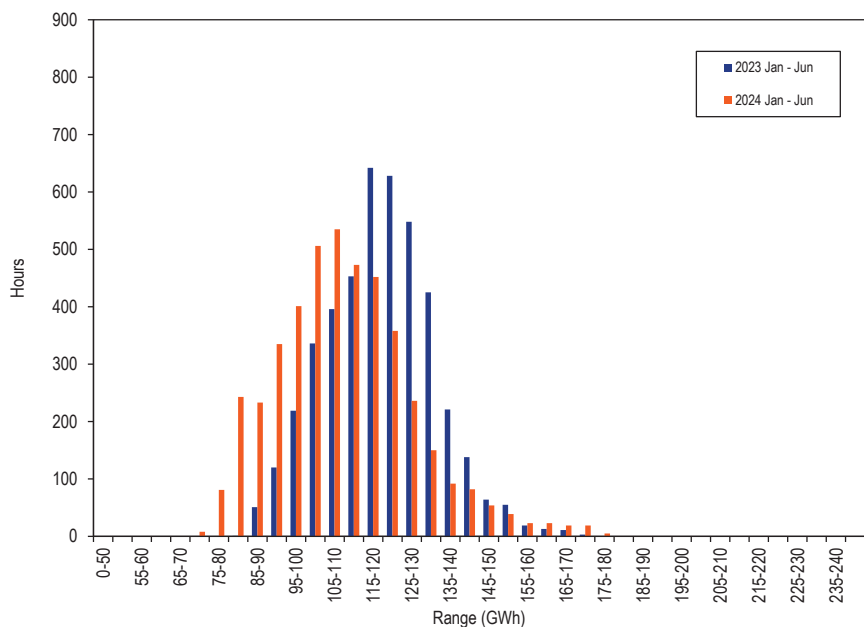
Figure 3-5 Distribution of day-ahead cleared supply plus imports: January through June, 2023 and 2024 28
