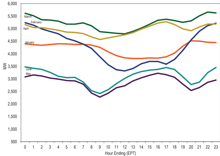
Figure 8-16 Average hourly real-time generation of wind units: January through June, 2024
