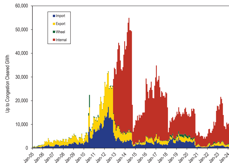
Figure 3-23 Monthly cleared up to congestion transactions by type (GWh): January 2005 through June 2024
