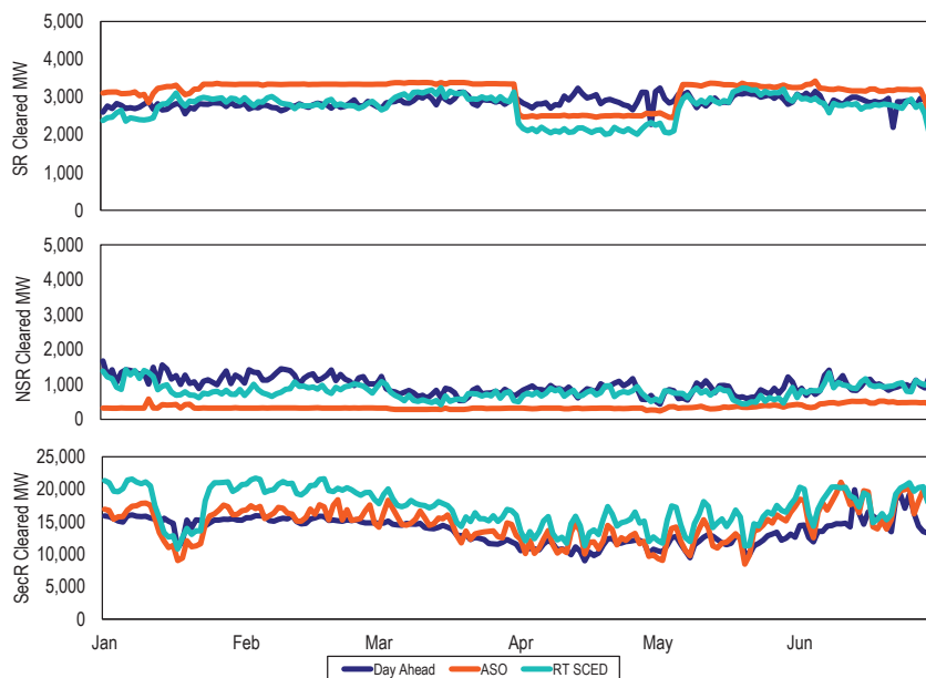
Figure 10-3 MW cleared by the day-ahead engine, the ASO, and RT SCED: January through June, 2024
