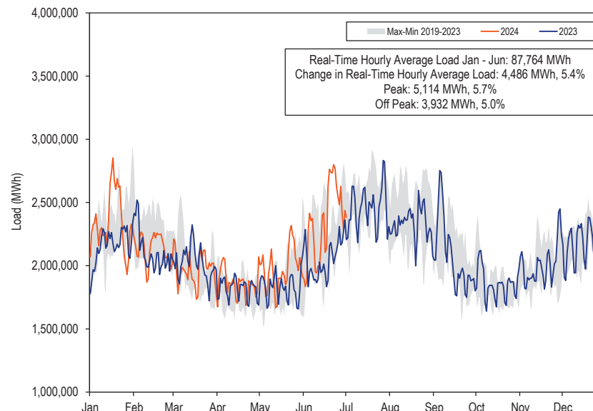
Figure 3-12 Real-time daily load: 2023 through June 2024
