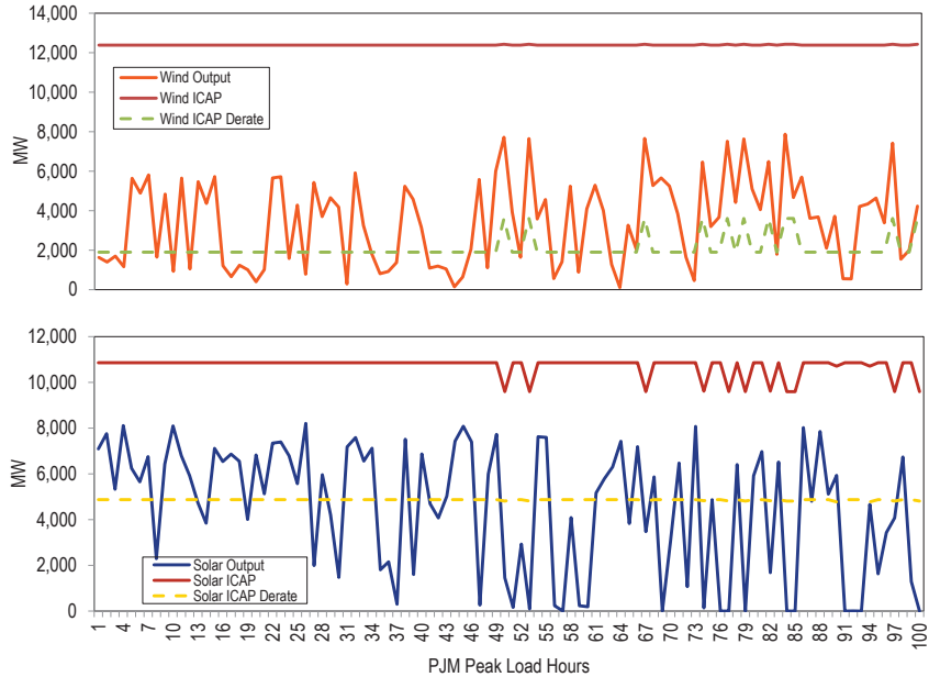
Figure 8-14 Wind and solar output during the top 100 load hours: January through June, 2024
