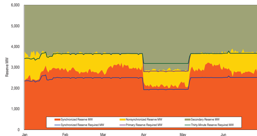
Figure 10-2 Daily average real-time reserve products cleared and daily average real-time reserve service requirements used by RT SCED: January through June, 2024
