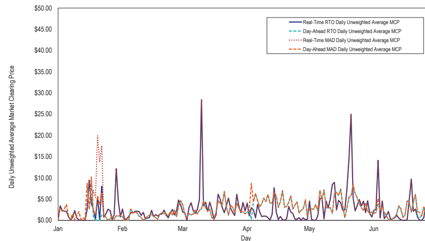
Figure 10-12 Day-ahead and real-time synchronized reserve average market clearing prices: January through June, 2024
