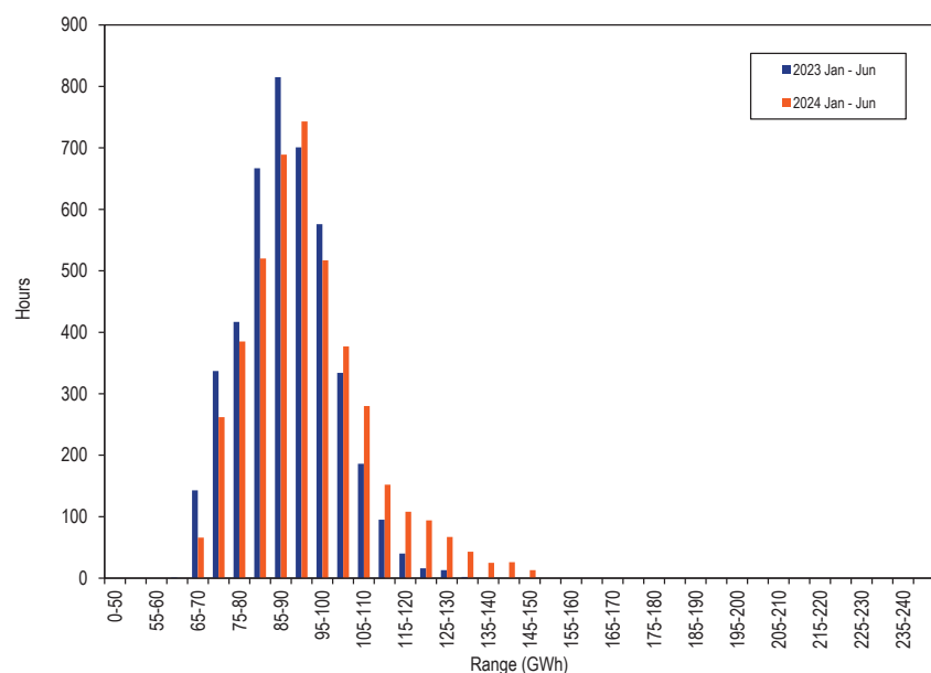
Figure 3-10 Distribution of real-time load plus exports: January through June, 2023 and 2024 36
