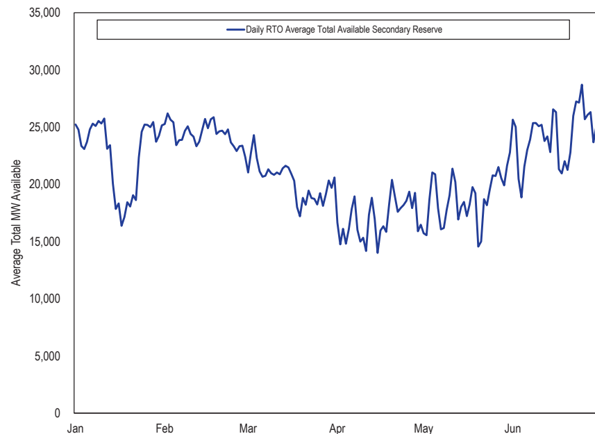
Figure 10-28 Daily Average Available Secondary Reserve: January through June, 2024
