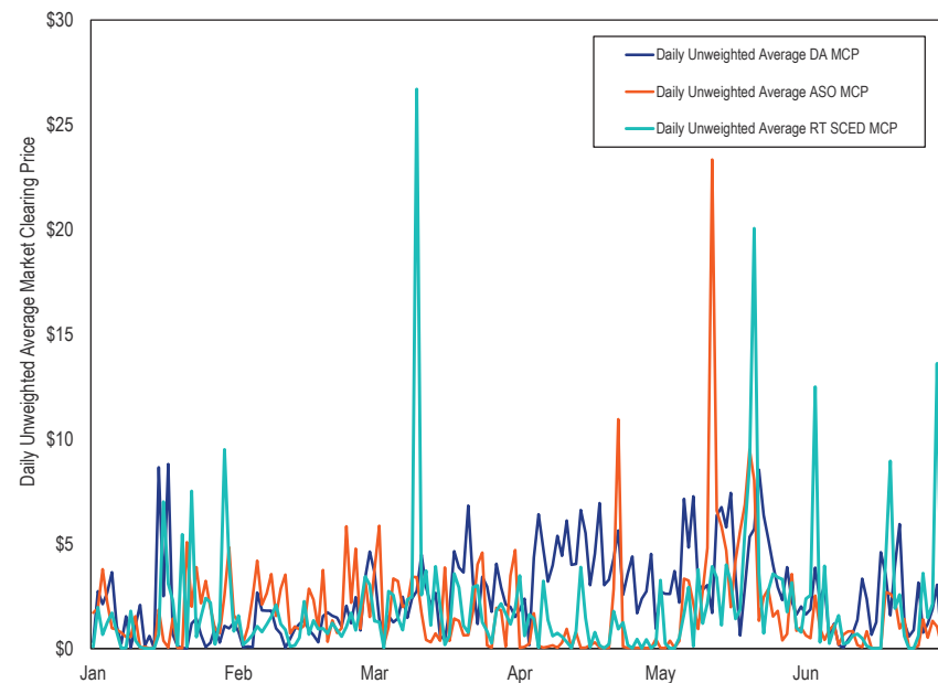
Figure 10-13 Dispatch run synchronized reserve market clearing prices from the day-ahead software, the ASO, and RT SCED: January through June, 2024
