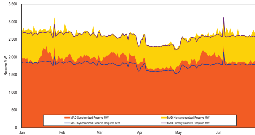
Figure 10-7 Daily average real-time MAD reserve products and daily average real-time MAD reserve service requirements: January through June, 2024
