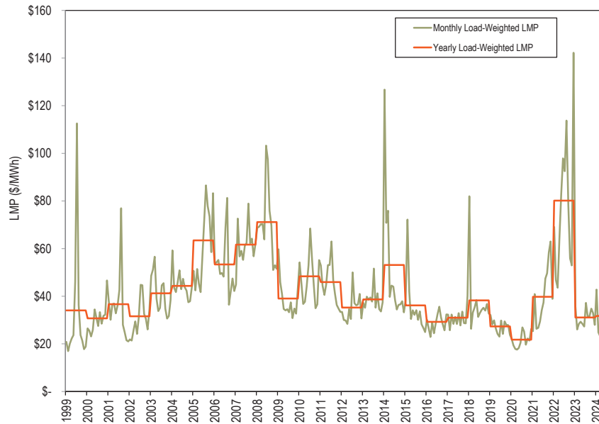
Figure 3-29 Real-time monthly and yearly load-weighted average LMP: 1999 through June 2024
