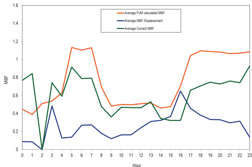
Figure 10-35 Effect of PJM's current dual offer clearing method on the average MBF in each hour of the day: January through June, 2024
