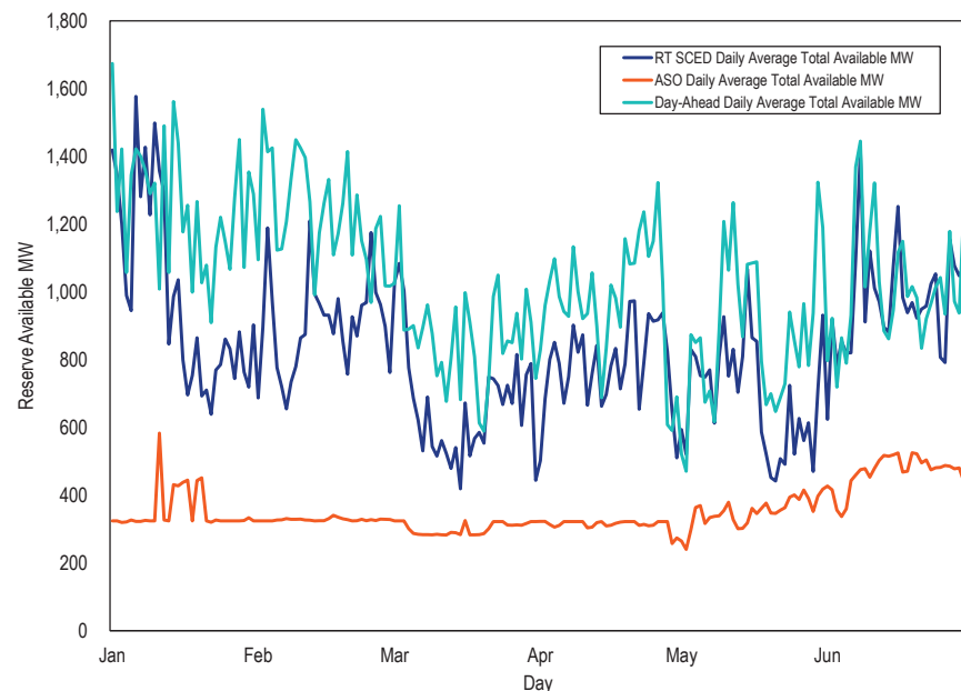
Figure 10-24 Daily average total available MW in the day-ahead, ASO, and RT SCED solutions: January through June, 2024
