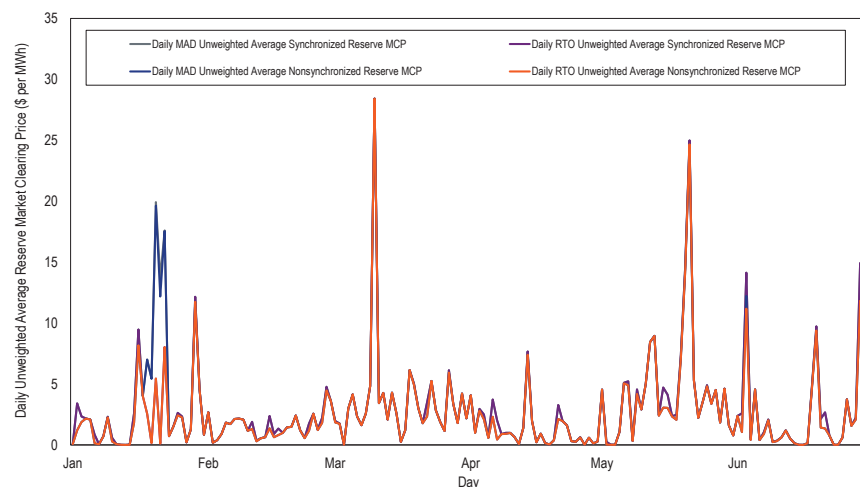
Figure 10-9 Daily average market clearing prices for synchronized reserve and nonsynchronized reserve: January through June, 2024
