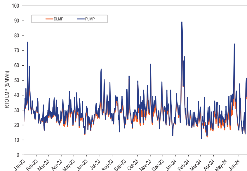
Figure 3-25 Real-time daily average DLMP and PLMP: 2023 through June 2024
