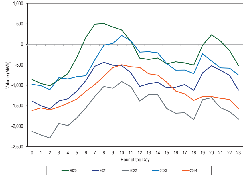
Figure 3-17 Difference between day-ahead and real-time hourly average load by hour of the day (Average hourly volumes): January through June, 2020 through 2024
