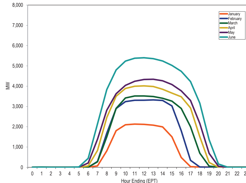
Figure 8-20 Average hourly day-ahead generation of solar units: January through June, 2024
