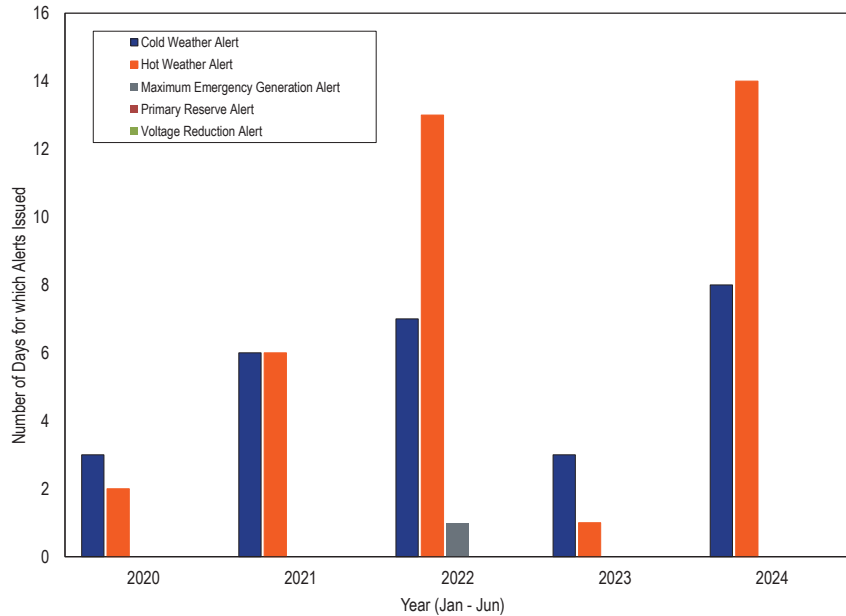
Figure 3-50 Number of days for which emergency alerts declared : January through June, 2020 through 2024
