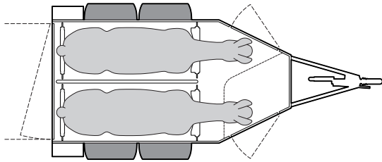
S80 With tack room 2 horses
