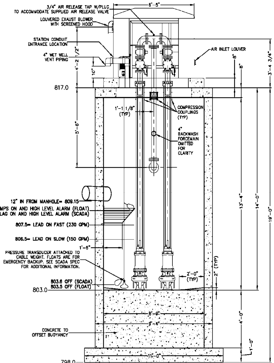
MUNTERS LIFT STATION FRONT SECTION
