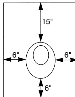
FHA SHAKE-ROOF FLASHING
