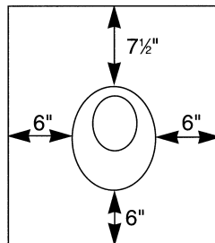
FHA FLASHING
