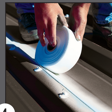
4 Reinforce existing seams with Spunflex® or Butyl Tape and base coat.
