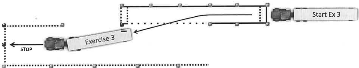
Figure 12.4: Step 4 – Reverse Offset Backing
