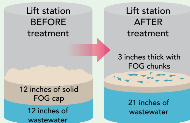
Figure 1: Solid FOG cap prior to treatment (left), digested and liquified FOG cap after two months of treatment (right)
