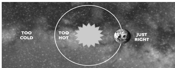
Earth orbits within the Habitable Zone of the Sun.
