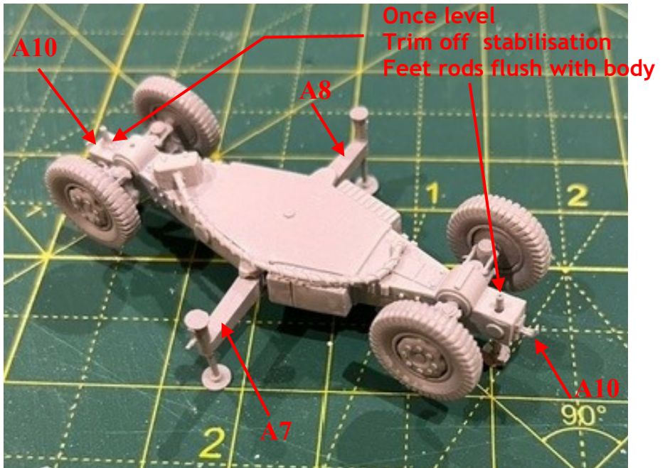
Phase 1 Completed in normal towing position
